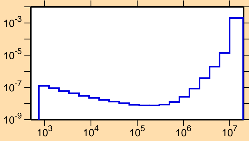
\sigma vs. E for ^{131}\text{Xe}(n,\alpha)
