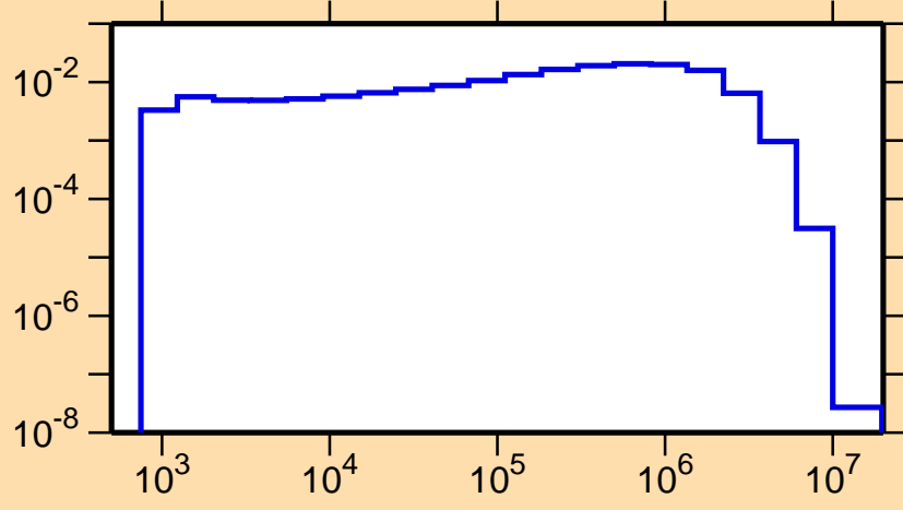
\sigma vs. E for ^{131}\text{Xe}(n,n_1)
