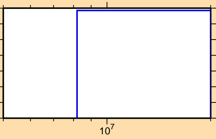
\sigma vs. E for ^{131}\text{Xe}(n,3n)
