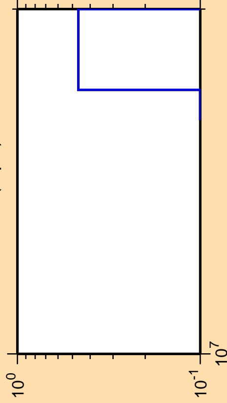
\Delta\sigma/\sigma vs. E for ^{132}\text{Xe}(n,p\alpha)
