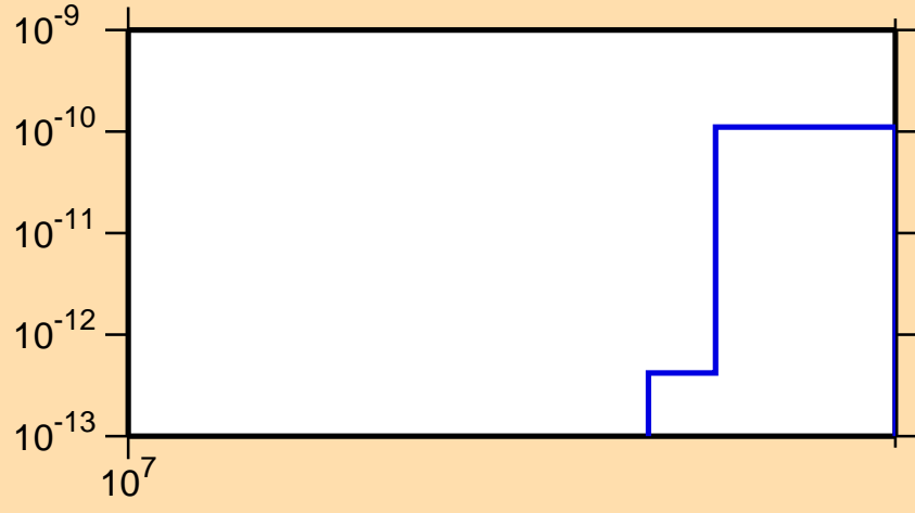
\sigma vs. E for ^{132}\text{Xe}(n,\text{He}3)
