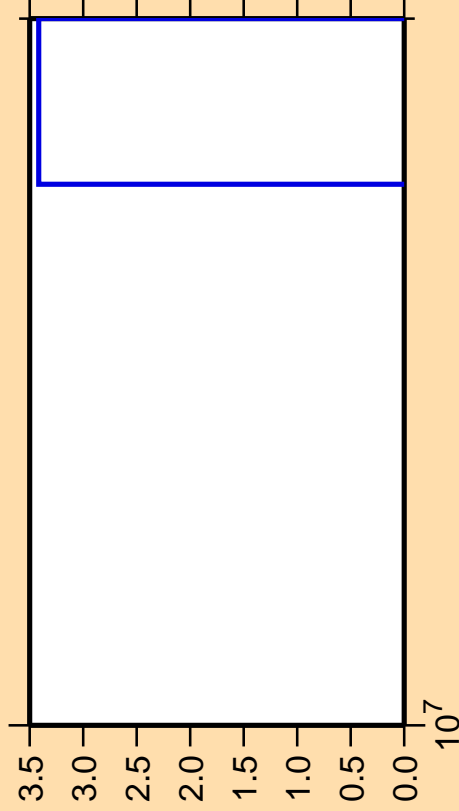
\Delta\sigma/\sigma vs. E for ^{132}\text{Xe}(n,2np)
