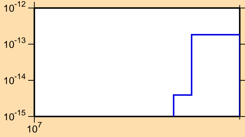
\sigma vs. E for ^{132}\text{Xe}(n,p\alpha)
