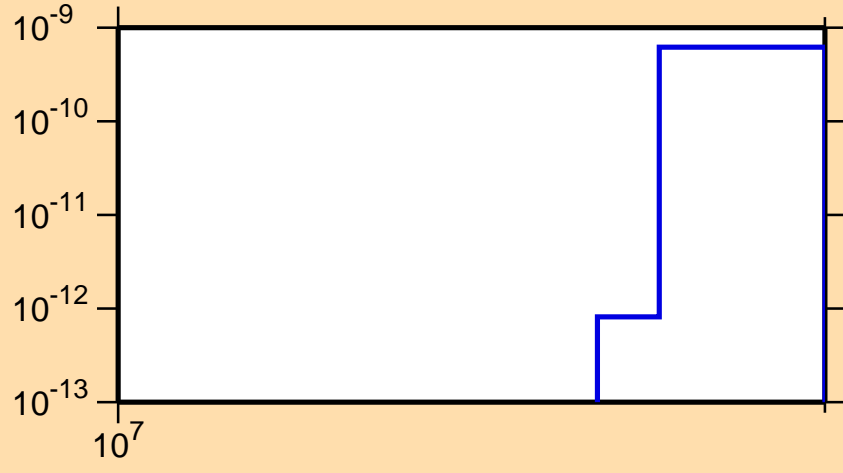
\sigma vs. E for ^{132}\text{Xe}(n,2n\alpha)
