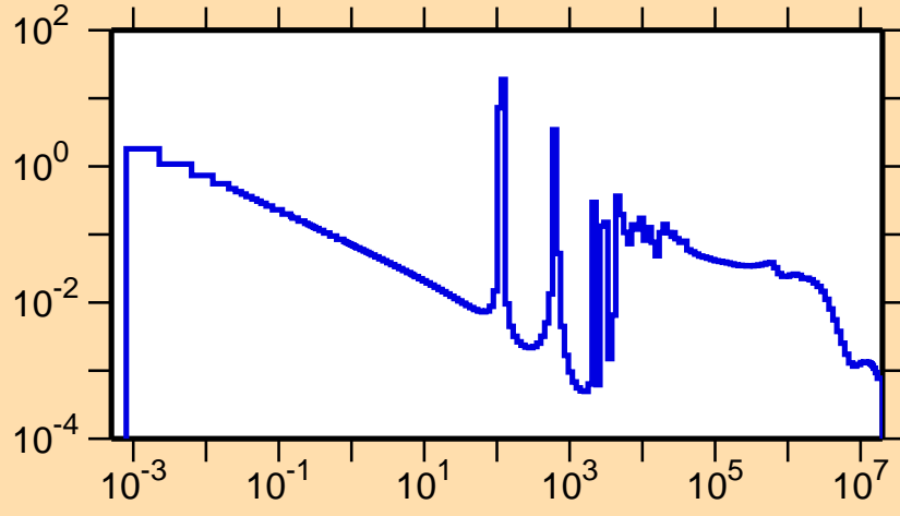
\sigma vs. E for ^{132}\text{Xe}(n,\gamma)
