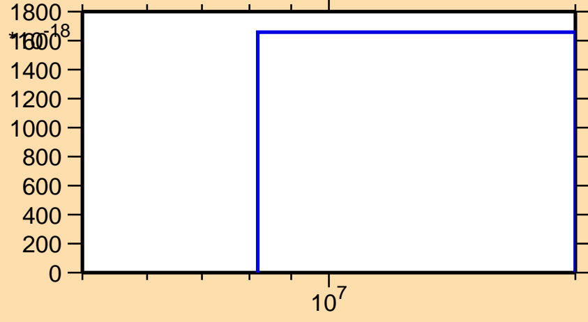
\sigma vs. E for ^{132}\text{Xe}(n,p\alpha)
