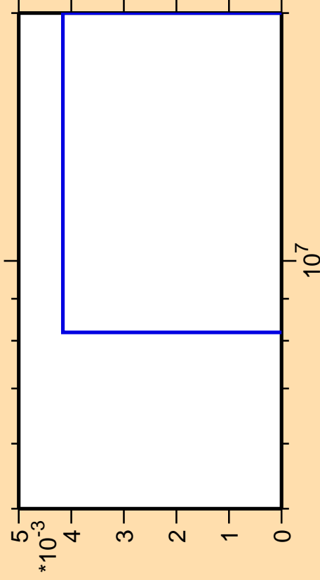
\Delta\sigma/\sigma vs. E for ^{132}\text{Xe}(n,p\alpha)
