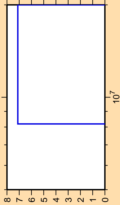
\Delta\sigma/\sigma vs. E for ^{132}\text{Xe}(n,2n\alpha)
