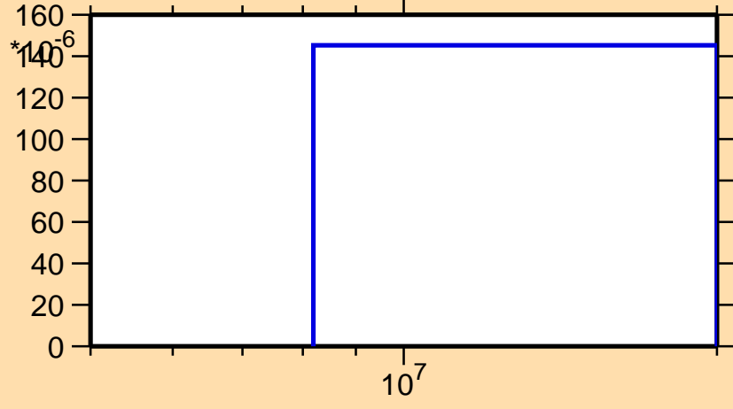
\sigma vs. E for ^{133}\text{Xe}(n,np)
