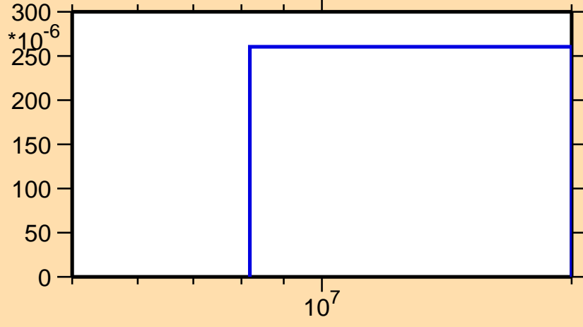
\sigma vs. E for ^{133}\text{Xe}(n,d)
