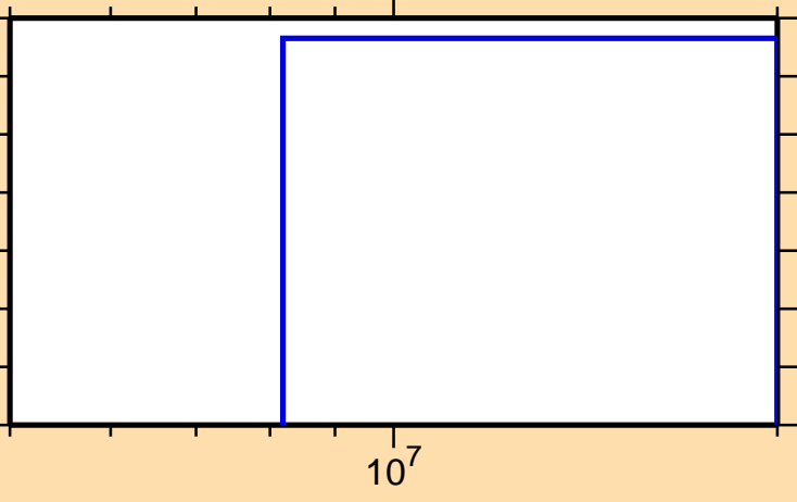
\sigma vs. E for ^{133}\text{Xe}(n,\text{nd})
