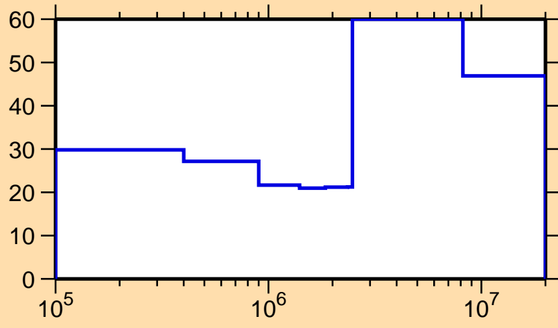
\Delta\sigma/\sigma vs. E for ^{133}\text{Xe}(n,n_1)
