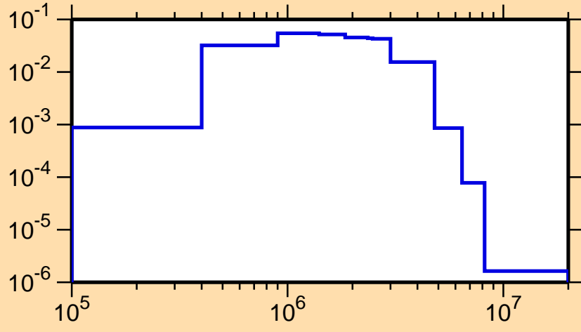
\sigma vs. E for ^{133}\text{Xe}(n,n_3)
