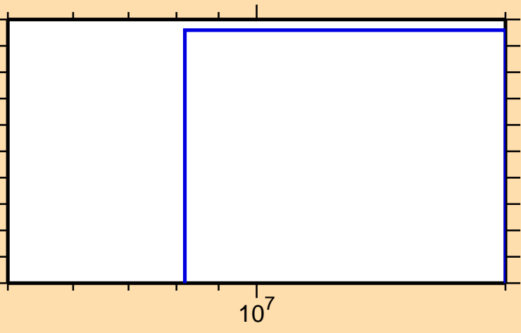
\sigma vs. E for ^{133}\text{Xe}(n,t)
