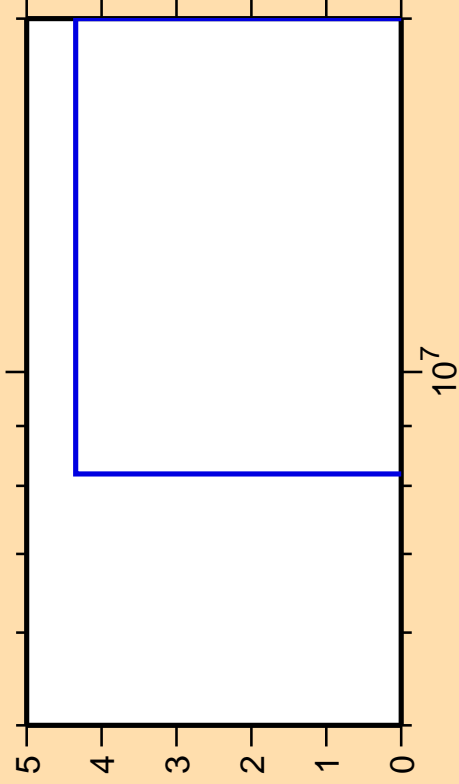
\Delta\sigma/\sigma vs. E for ^{134}\text{Xe}(n,2n\alpha)
