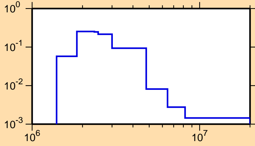
\sigma vs. E for ^{134}\text{Xe}(n,n_2)
