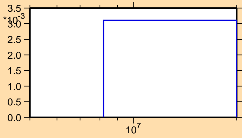
\sigma vs. E for ^{134}\text{Xe}(n,3n)
