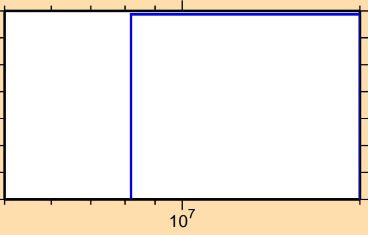
\sigma vs. E for ^{134}\text{Xe}(n,nt)
