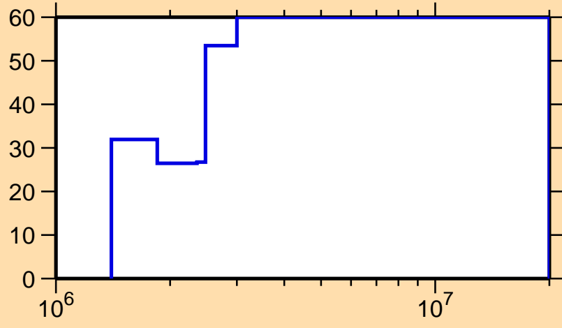
\Delta\sigma/\sigma vs. E for ^{134}\text{Xe}(n,n_1)
