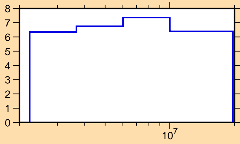
\Delta\sigma/\sigma vs. E for ^{135}\text{Xe}(n, n_{\text{nonel}})
