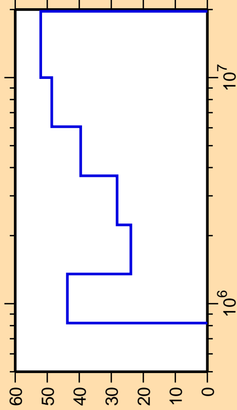
\Delta\sigma/\sigma vs. E for ^{135}\text{Xe}(n,n_4)
