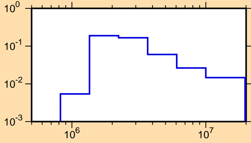
\sigma vs. E for ^{135}\text{Xe}(n,n_4)
