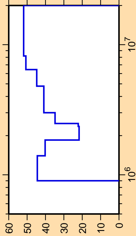
\Delta\sigma/\sigma vs. E for ^{135}\text{Xe}(n,n_3)
