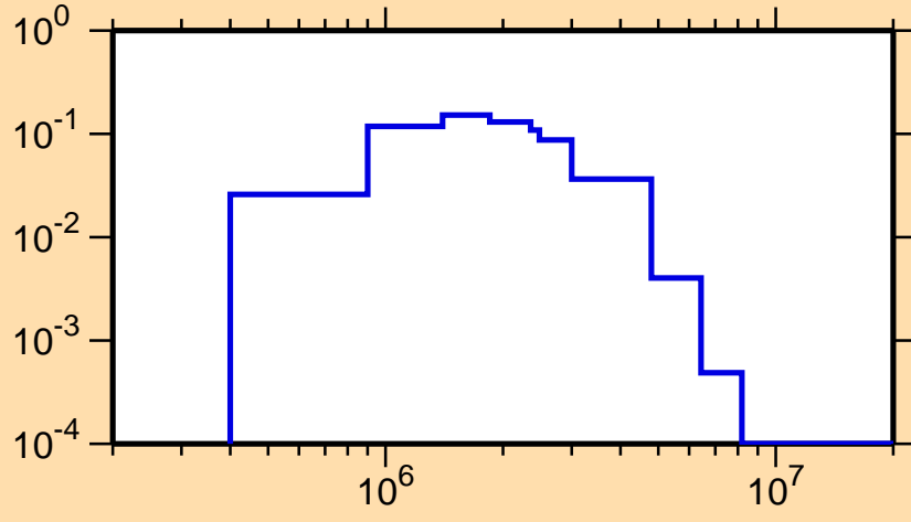
\sigma vs. E for ^{135}\text{Xe}(n,n_2)
