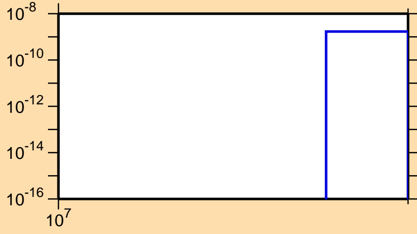
\sigma vs. E for ^{135}\text{Xe}(n,nt)
