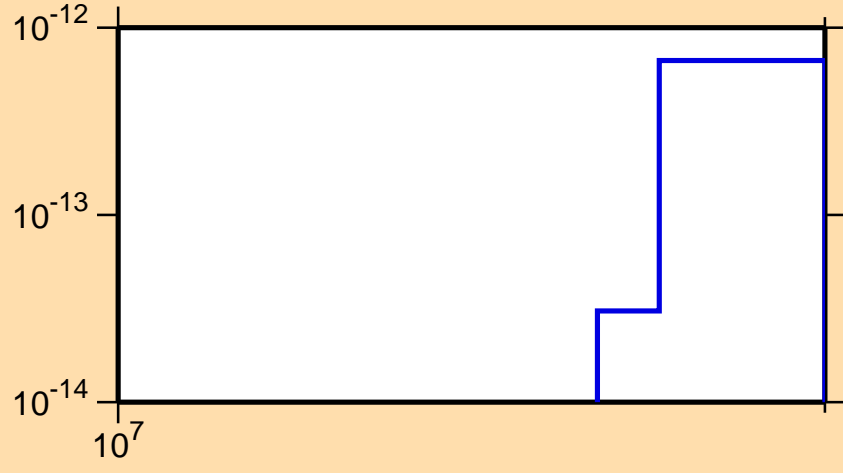
\sigma vs. E for ^{135}\text{Xe}(n,p\alpha)
