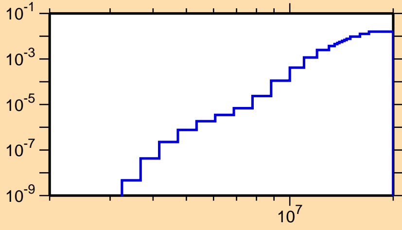
\sigma vs. E for ^{135}\text{Xe}(n,p)
