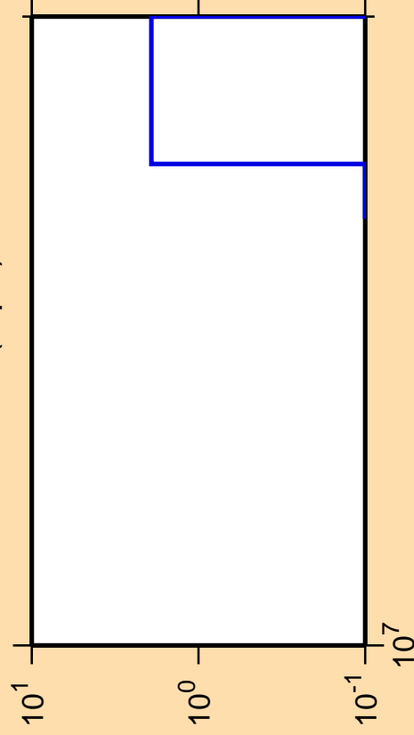
\Delta\sigma/\sigma vs. E for ^{135}\text{Xe}(n,p\alpha)
