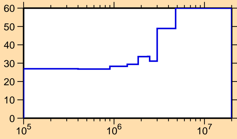
\Delta\sigma/\sigma vs. E for ^{135}\text{Xe}(n,\gamma)
