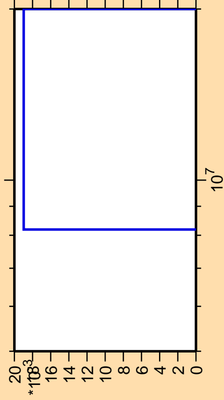
\Delta\sigma/\sigma vs. E for ^{135}\text{Xe}(n,p\alpha)
