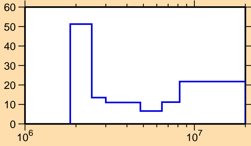
\Delta\sigma/\sigma vs. E for ^{135}\text{Xe}(n,n\text{cont.})
