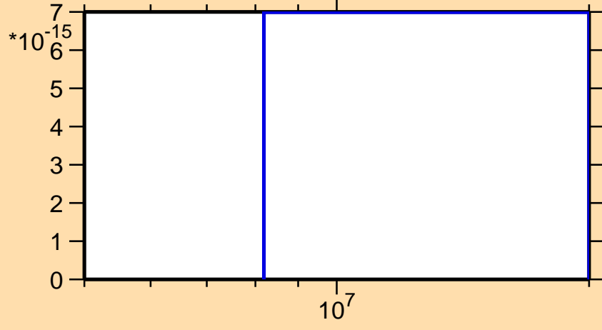
\sigma vs. E for ^{135}\text{Xe}(n,p\alpha)
