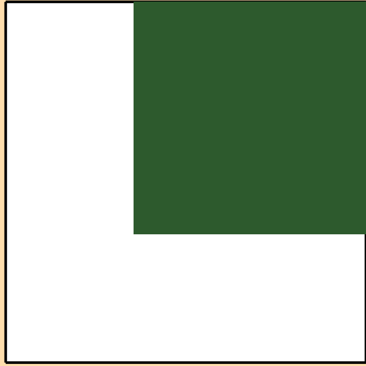
\sigma vs. E for ^{135}\text{Xe}(n,t)
