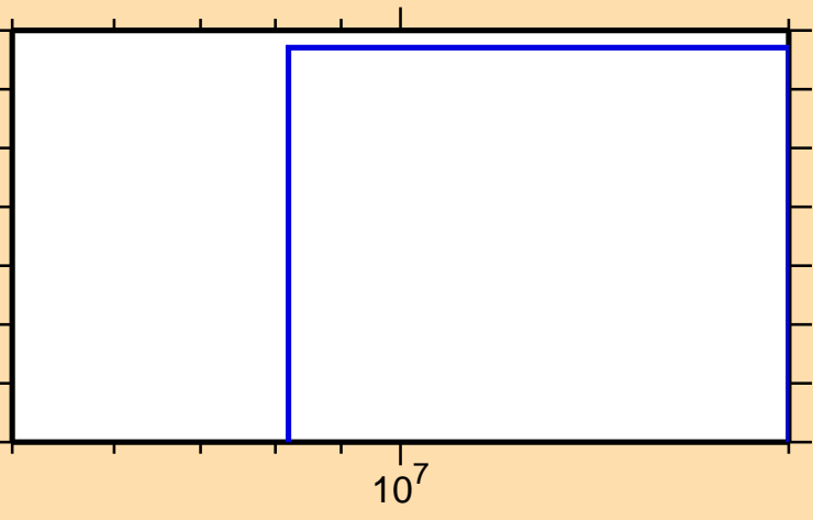
\sigma vs. E for ^{135}\text{Xe}(n,t)
