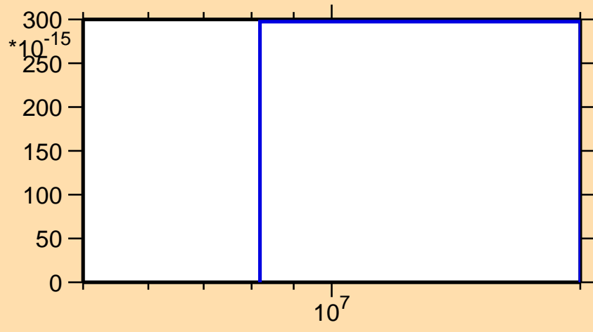
\sigma vs. E for ^{136}\text{Xe}(n,2n\alpha)
