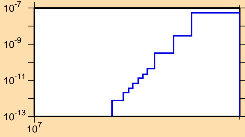
\sigma vs. E for ^{137}\text{Xe}(n,2n\alpha)
