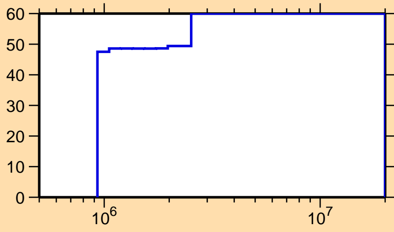
\Delta\sigma/\sigma vs. E for ^{138}\text{Xe}(n,\gamma)
