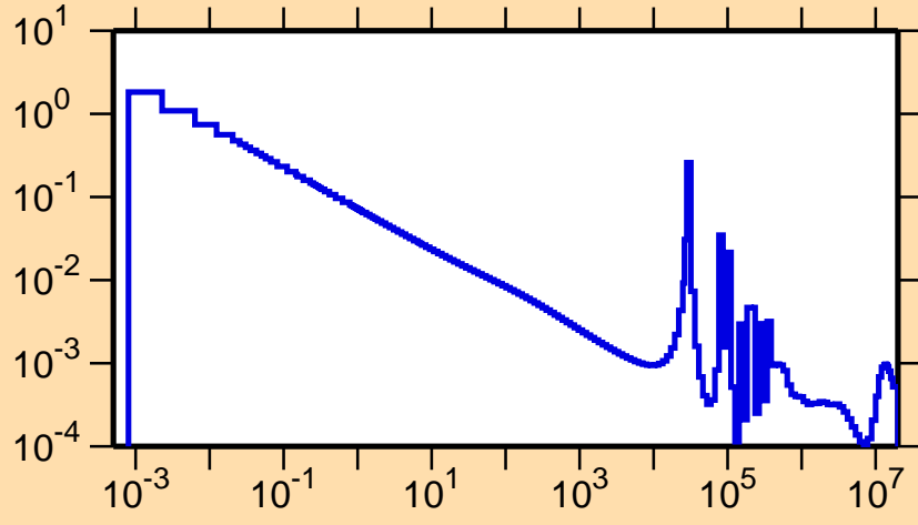
\sigma vs. E for ^{138}\text{Xe}(n,\gamma)
