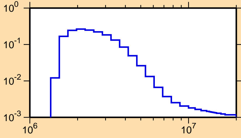
\sigma vs. E for ^{138}\text{Xe}(n,n_3)
