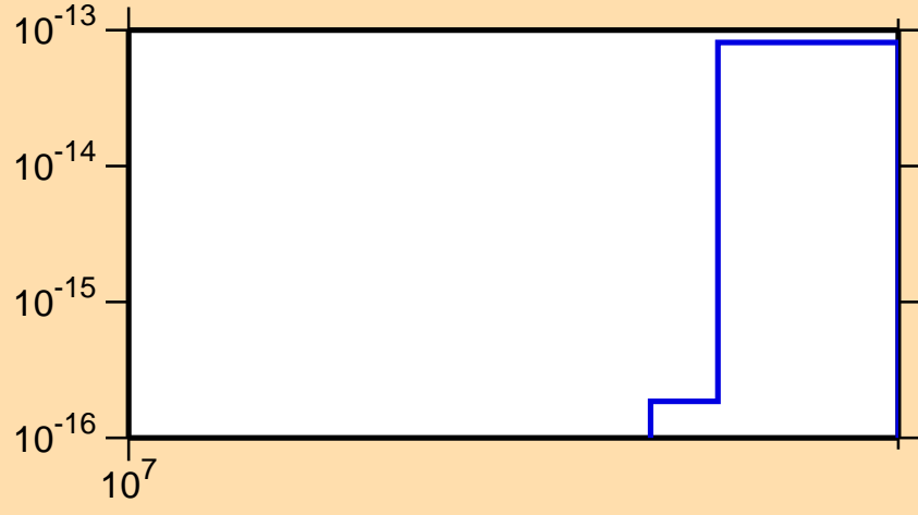
\sigma vs. E for ^{138}\text{Xe}(\text{mt117})
