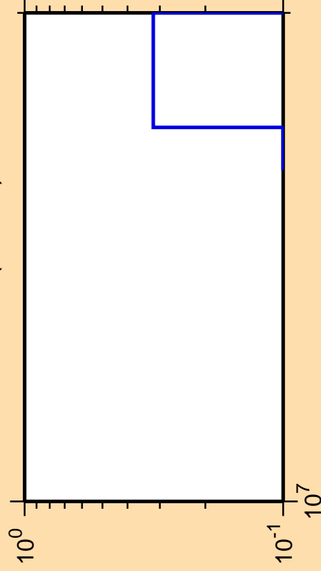
\Delta\sigma/\sigma vs. E for ^{138}\text{Xe}(\text{mt117})
