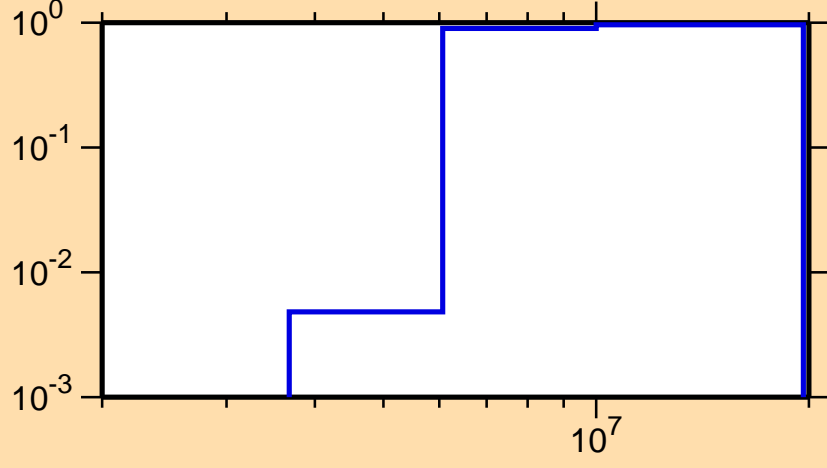
\sigma vs. E for ^{138}\text{Xe}(n,2n)
