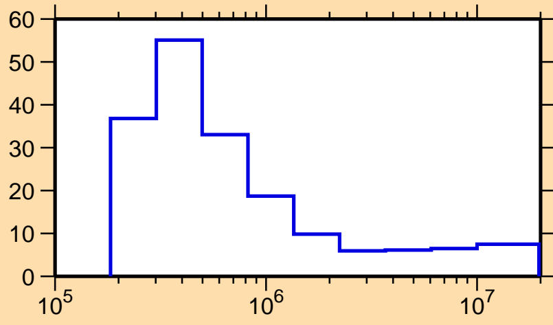
\Delta\sigma/\sigma vs. E for ^{138}\text{Xe}(n,\text{nonel.})
