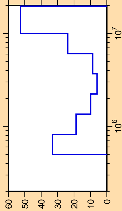
\Delta\sigma/\sigma vs. E for ^{138}\text{Xe}(n,\text{inel.})
