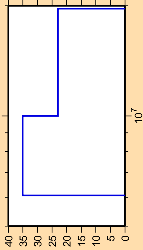
\Delta\sigma/\sigma vs. E for ^{138}\text{Xe}(n,3n)
