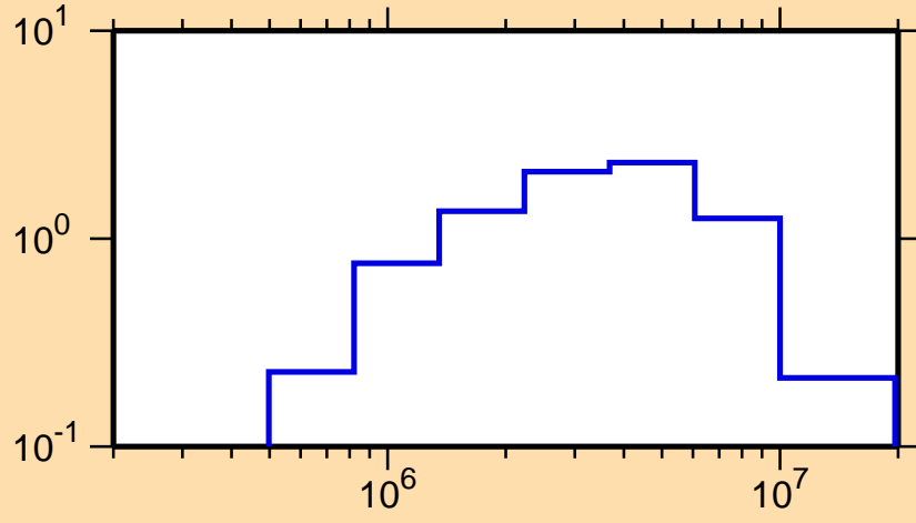
\sigma vs. E for ^{138}\text{Xe}(n,\text{inel.})
