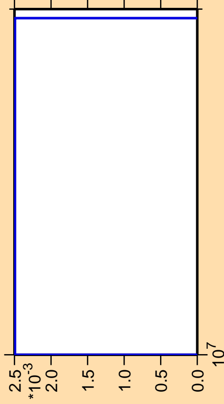
\Delta\sigma/\sigma vs. E for ^{138}\text{Xe}(\text{mt117})
