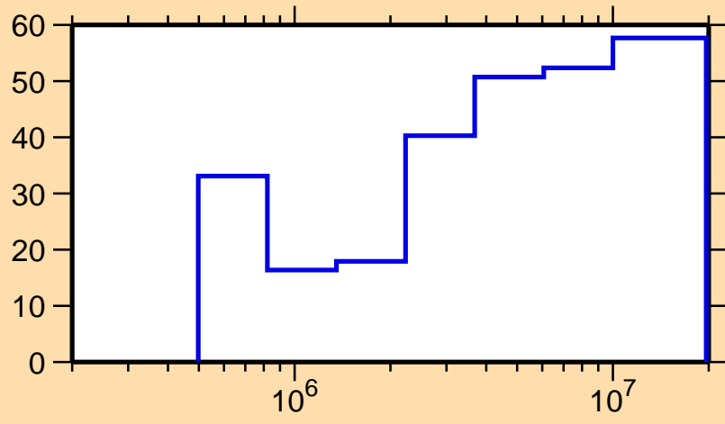
\Delta\sigma/\sigma vs. E for ^{138}\text{Xe}(n,n_1)
