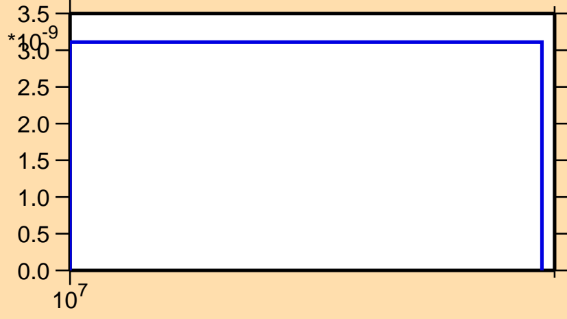
\sigma vs. E for ^{138}\text{Xe}(n,2n\alpha)
