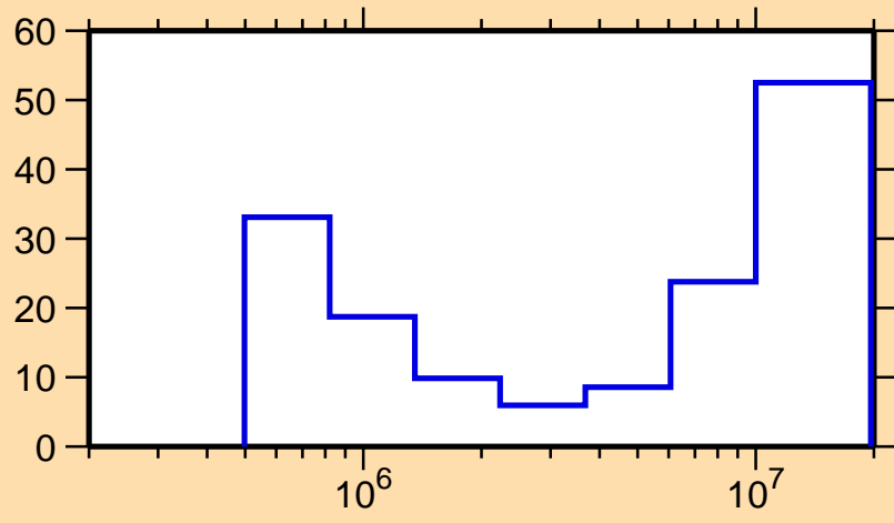
\Delta\sigma/\sigma vs. E for ^{138}\text{Xe}(n,\text{inel.})
