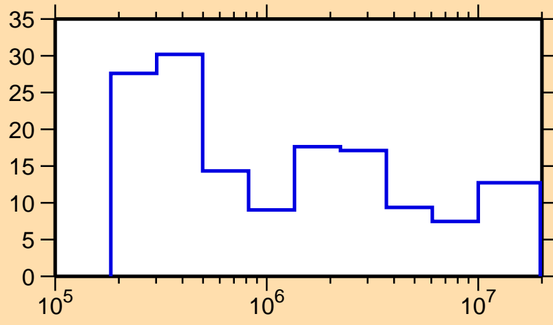
\Delta\sigma/\sigma vs. E for ^{138}\text{Xe}(n,\text{el.})
