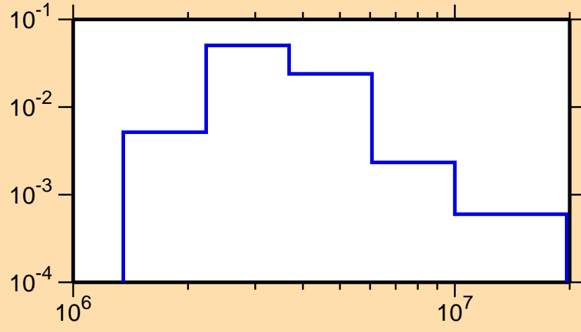
\sigma vs. E for ^{138}\text{Xe}(n,n_4)
