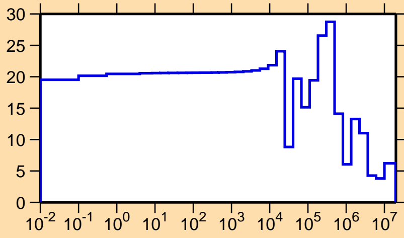
\Delta\sigma/\sigma vs. E for ^{138}\text{Xe}(n,\text{tot.})
