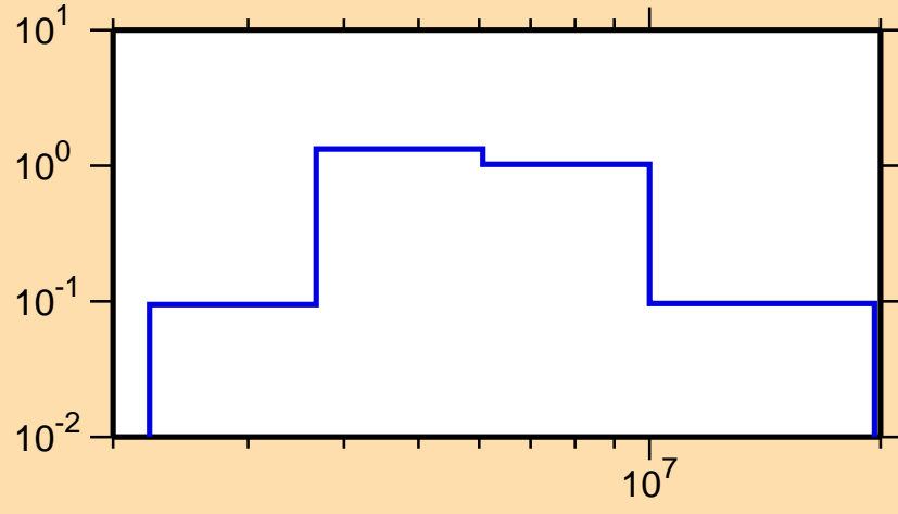
\sigma vs. E for ^{138}\text{Xe}(n,n\text{cont.})
