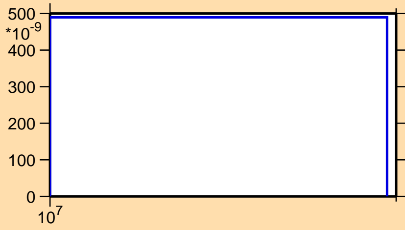
\sigma vs. E for ^{138}\text{Xe}(n,nt)
