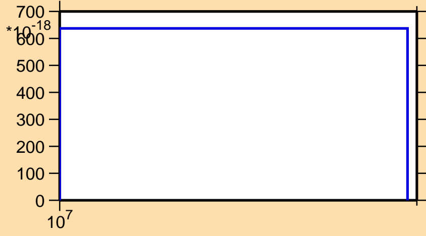
\sigma vs. E for ^{138}\text{Xe}(\text{mt117})
