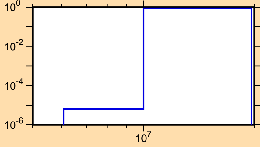
\sigma vs. E for ^{138}\text{Xe}(n,3n)
