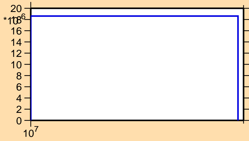
\sigma vs. E for ^{138}\text{Xe}(n,d)
