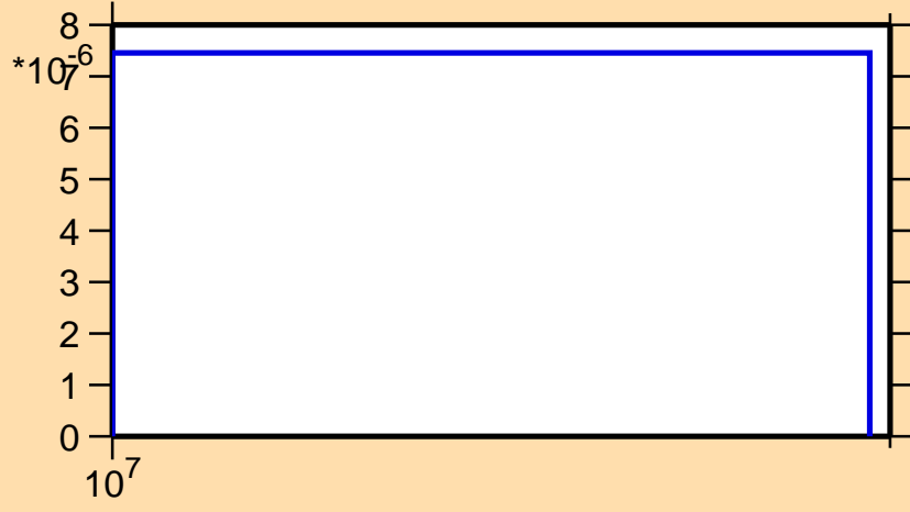
\sigma vs. E for ^{138}\text{Xe}(n,np)
