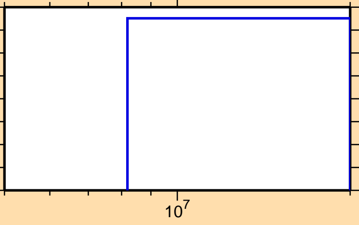
\sigma vs. E for ^{138}\text{Xe}(n,d)
