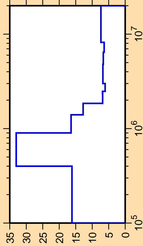
\Delta\sigma/\sigma vs. E for ^{138}\text{Xe}(n,\text{nonel.})
