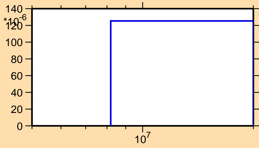
\sigma vs. E for ^{138}\text{Xe}(n,p)
