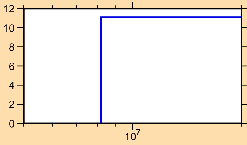
\Delta\sigma/\sigma vs. E for ^{138}\text{Xe}(n,el.)
