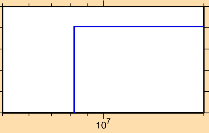
\sigma vs. E for ^{138}\text{Xe}(n,t)
