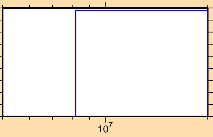
\sigma vs. E for ^{138}\text{Xe}(n,2np)
