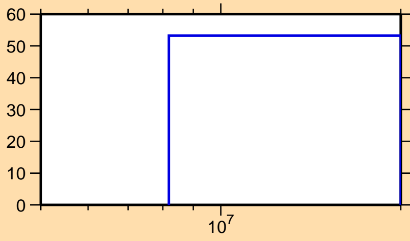
\Delta\sigma/\sigma vs. E for ^{138}\text{Xe}(n,n\text{cont.})
