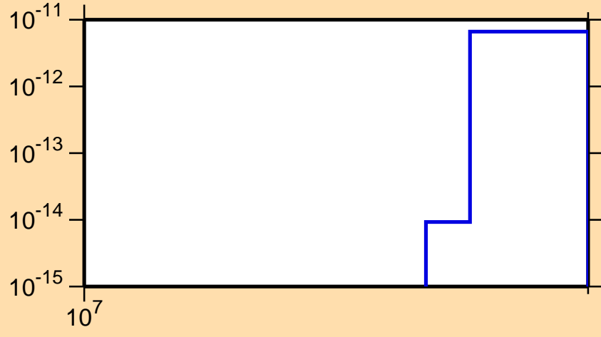
\sigma vs. E for ^{139}\text{Xe}(n,3n\alpha)
