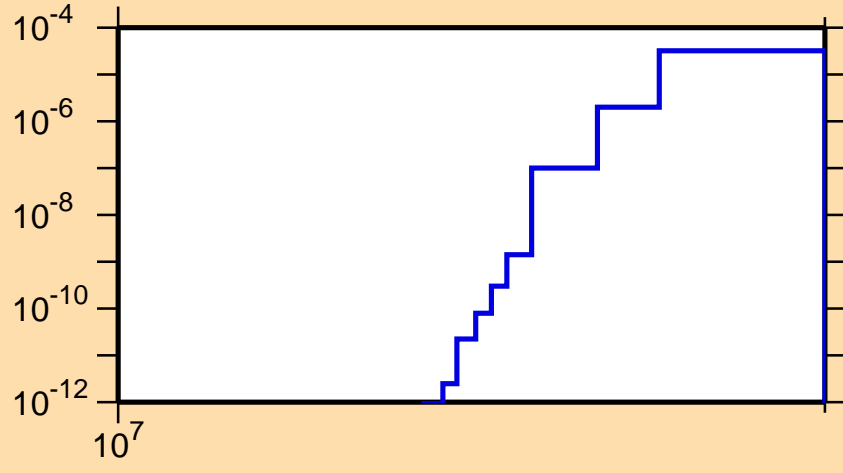
\sigma vs. E for ^{139}\text{Xe}(n,nt)
