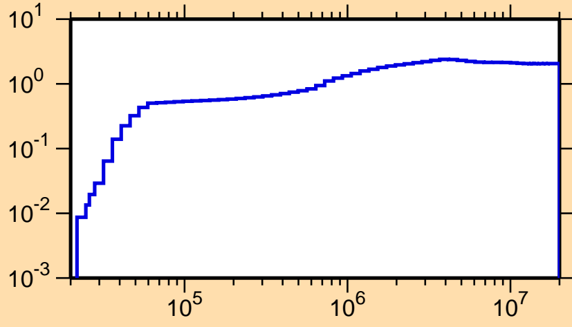
\sigma vs. E for ^{139}\text{Xe}(n,\text{nonel.})
