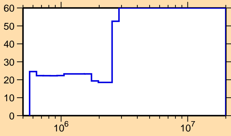
\Delta\sigma/\sigma vs. E for ^{139}\text{Xe}(n,n_1)
