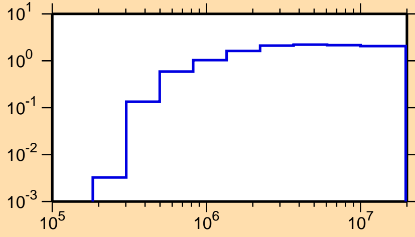
\sigma vs. E for ^{140}\text{Xe}(n,\text{nonel.})
