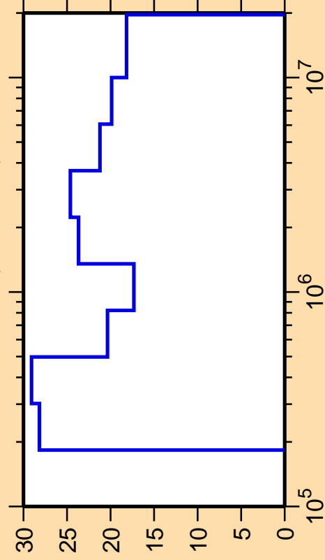
\Delta\sigma/\sigma vs. E for ^{140}\text{Xe}(n,\text{nonel.})
