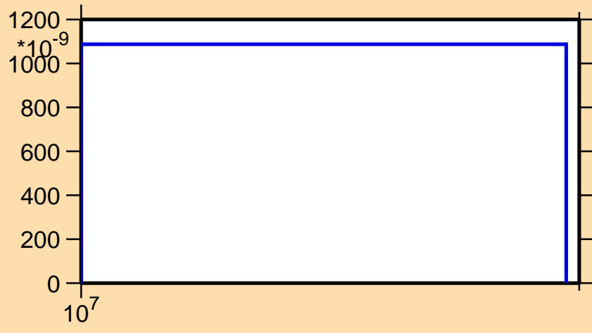
\sigma vs. E for ^{140}\text{Xe}(n,np)
