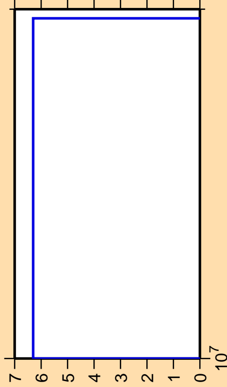
\Delta\sigma/\sigma vs. E for ^{140}\text{Xe}(n,2np)
