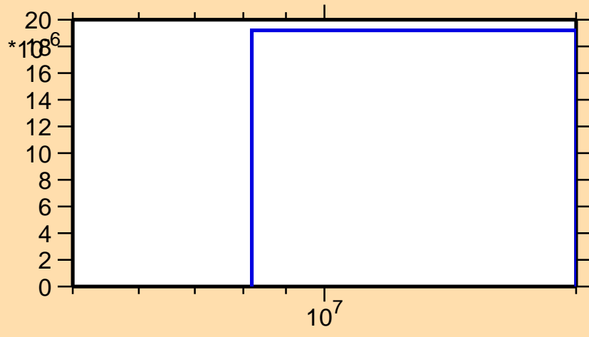
\sigma vs. E for ^{140}\text{Xe}(n,t)
