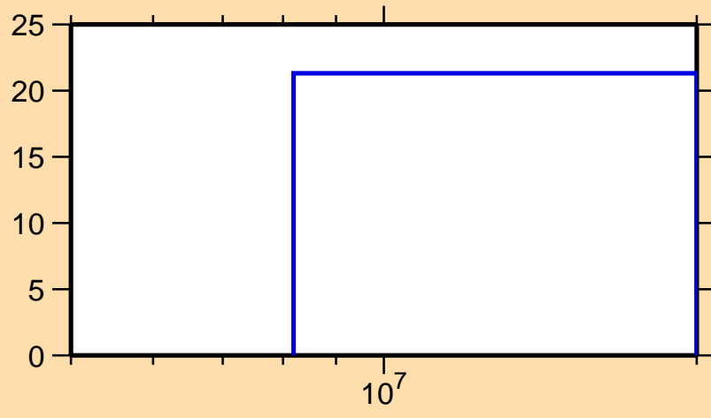
\Delta\sigma/\sigma vs. E for ^{140}\text{Xe}(n,el.)
