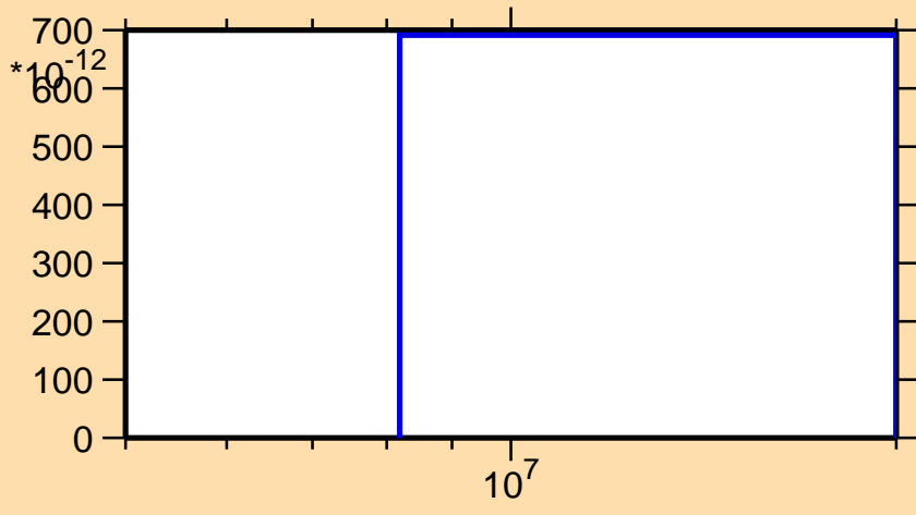
\sigma vs. E for ^{140}\text{Xe}(n,\text{nd})
