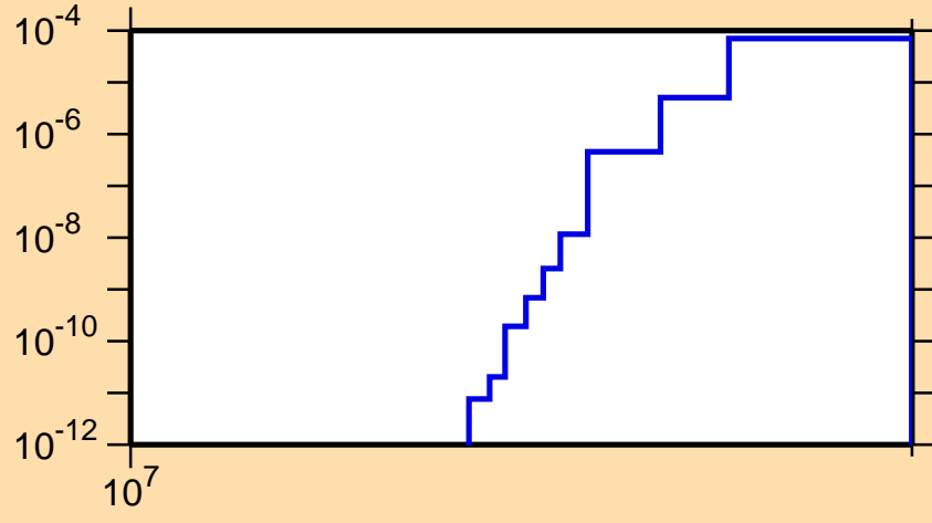
\sigma vs. E for ^{141}\text{Xe}(n,np)
