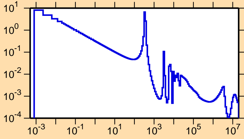
\sigma vs. E for ^{141}\text{Xe}(n,\gamma)
