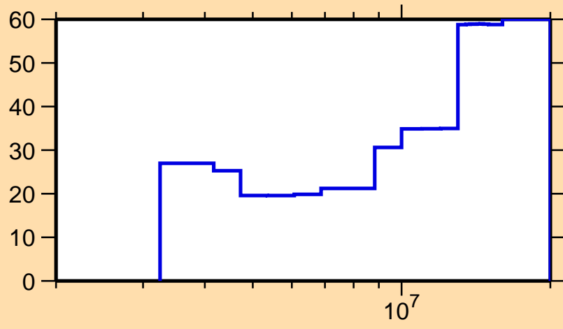
\Delta\sigma/\sigma vs. E for ^{141}\text{Xe}(n,2n)
