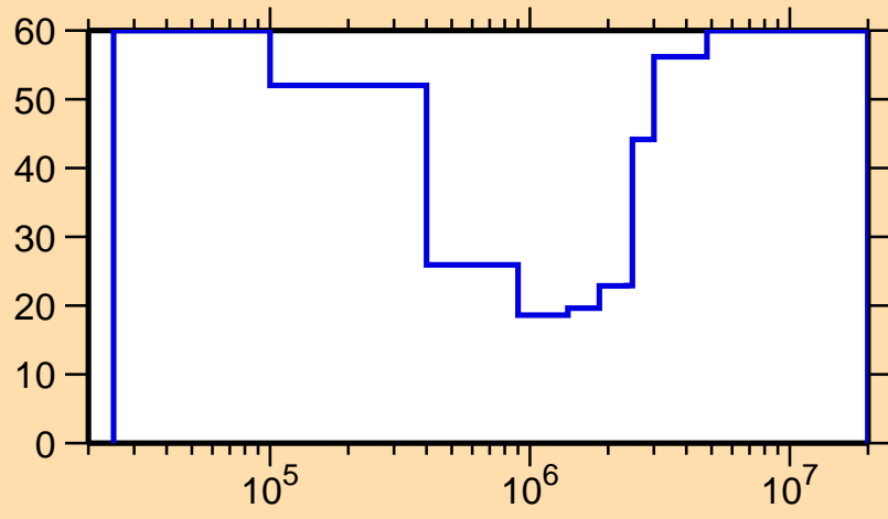
\Delta\sigma/\sigma vs. E for ^{141}\text{Xe}(n,n_1)
