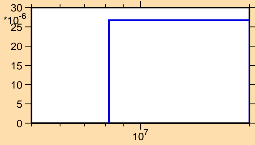
\sigma vs. E for ^{141}\text{Xe}(n,t)
