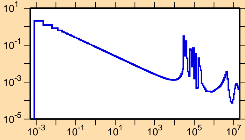
\sigma vs. E for ^{142}\text{Xe}(n,\gamma)
