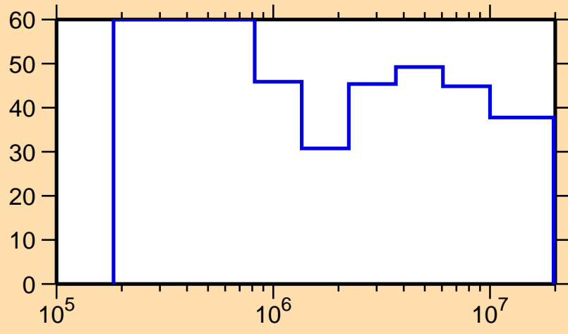
\Delta\sigma/\sigma vs. E for ^{142}\text{Xe}(n,n_1)
