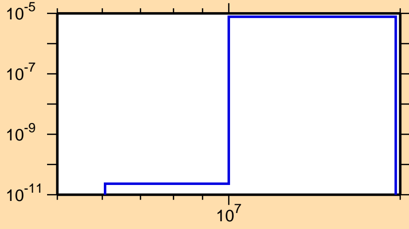
\sigma vs. E for ^{142}\text{Xe}(n,n\alpha)
