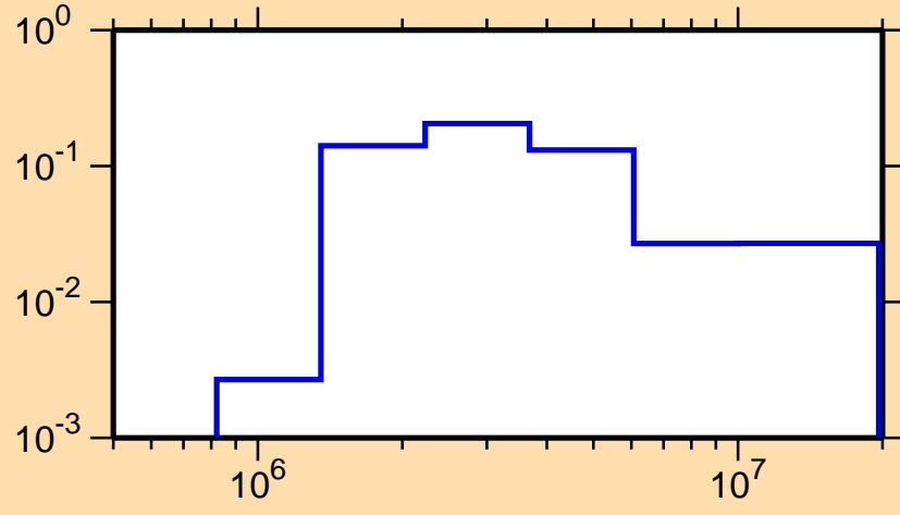
\sigma vs. E for ^{142}\text{Xe}(n,n_4)
