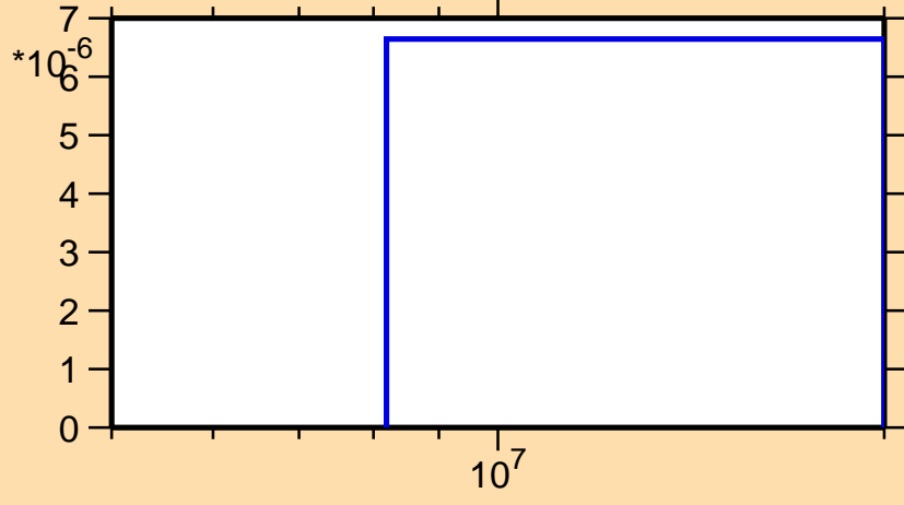
\sigma vs. E for ^{142}\text{Xe}(n,t)
