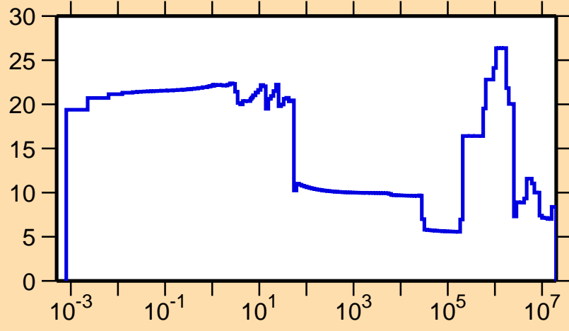
\Delta\sigma/\sigma vs. E for ^{78}\text{Y}(n,\text{el.})
