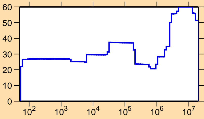
\Delta\sigma/\sigma vs. E for ^{78}\text{Y}(n,p)
