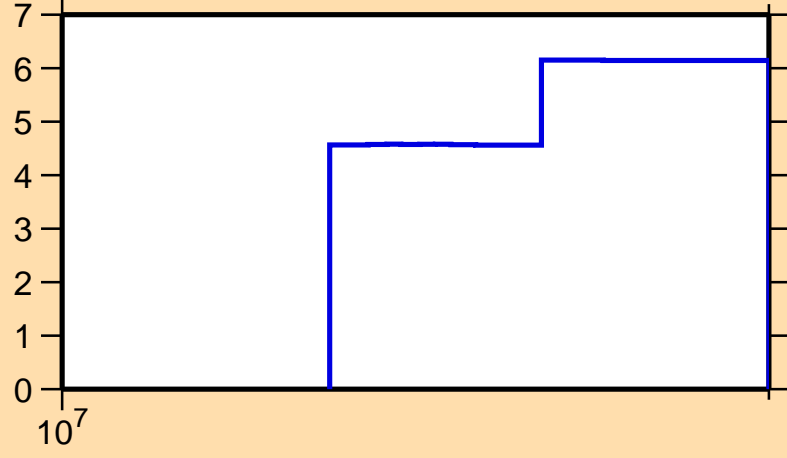
\Delta\sigma/\sigma vs. E for ^{78}\text{Y}(n,\text{tot.})
