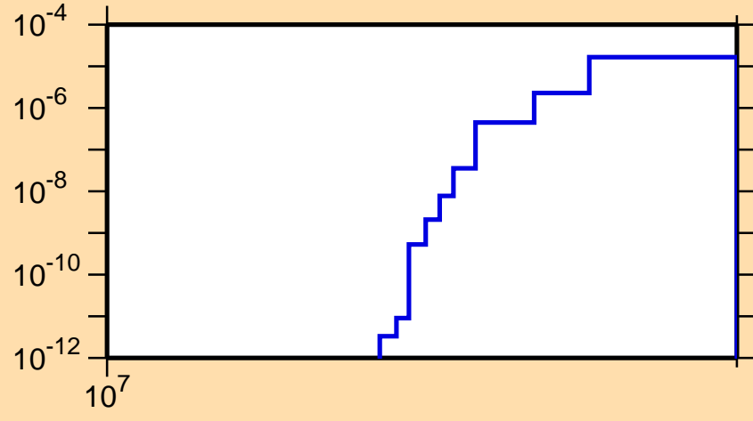
\sigma vs. E for ^{78}\text{Y}(n,2np)
