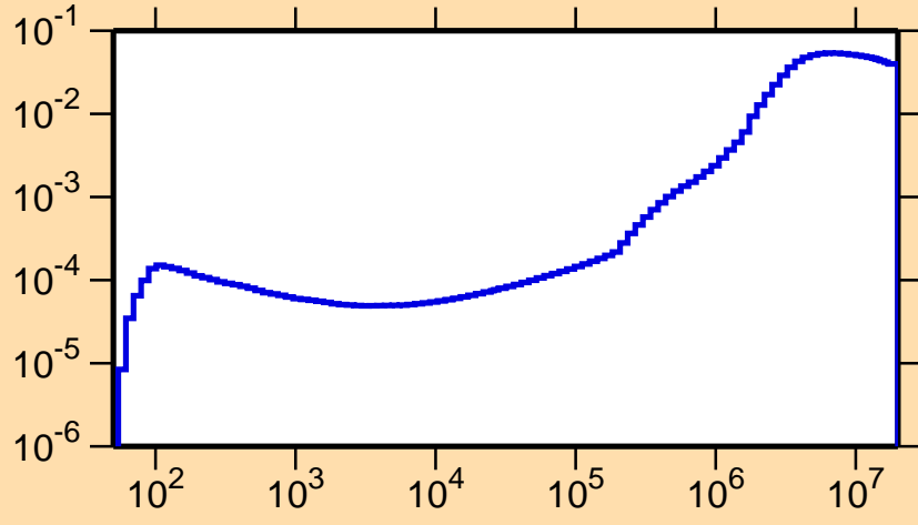
\sigma vs. E for ^{78}\text{Y}(n,\text{inel.})
