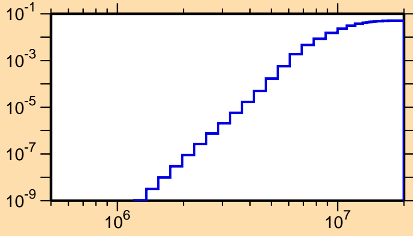
\sigma vs. E for ^{78}\text{Y}(n,d)
