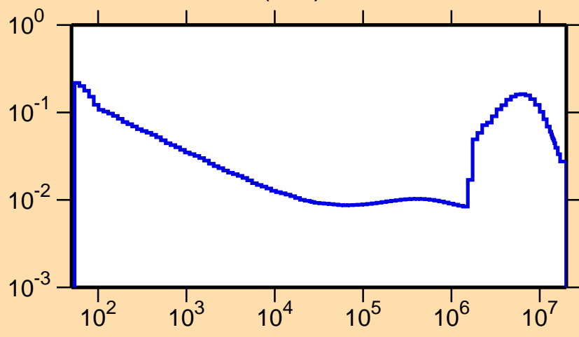
\sigma vs. E for ^{78}\text{Y}(n,\alpha)
