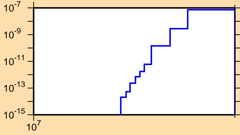
\sigma vs. E for ^{78}\text{Y} (mt 34)
