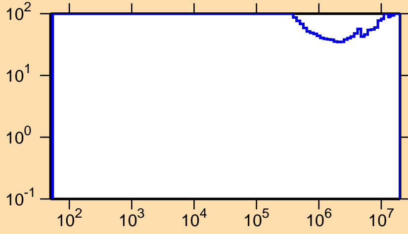
\Delta\sigma/\sigma vs. E for ^{78}\text{Y}(n,n_1)
