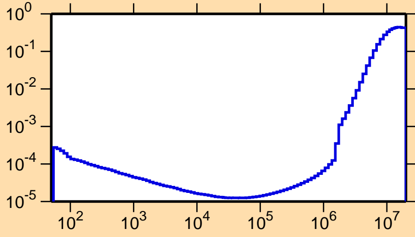
\sigma vs. E for ^{78}\text{Y}(n,p\alpha)
