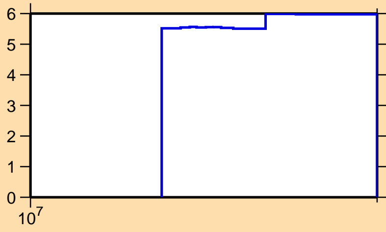
\Delta\sigma/\sigma vs. E for ^{78}\text{Y}(n,\text{nonel.})
