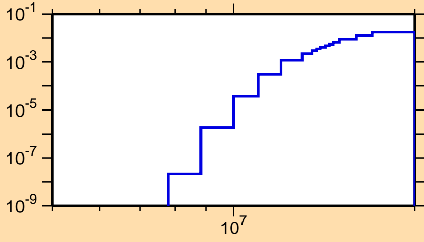
\sigma vs. E for ^{78}\text{Y}(n,pd)
