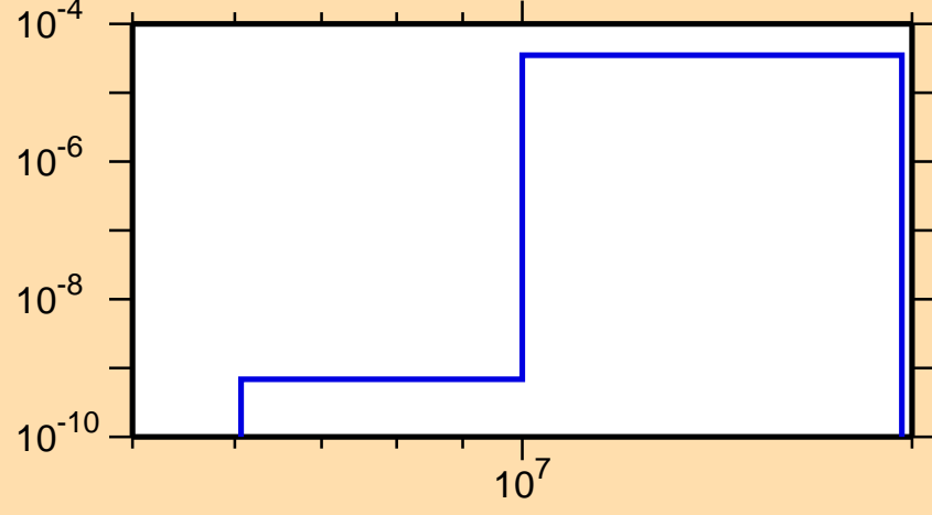
\sigma vs. E for ^{78}\text{Y}(n,n\alpha)
