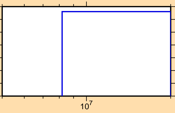
\sigma vs. E for ^{78}\text{Y}(n,\text{pt})
