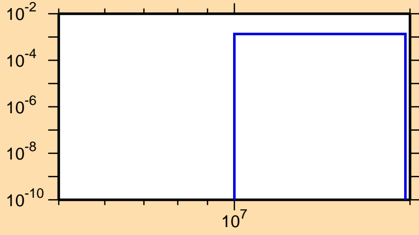
\sigma vs. E for ^{79}\text{Y}(n,\text{pd})
