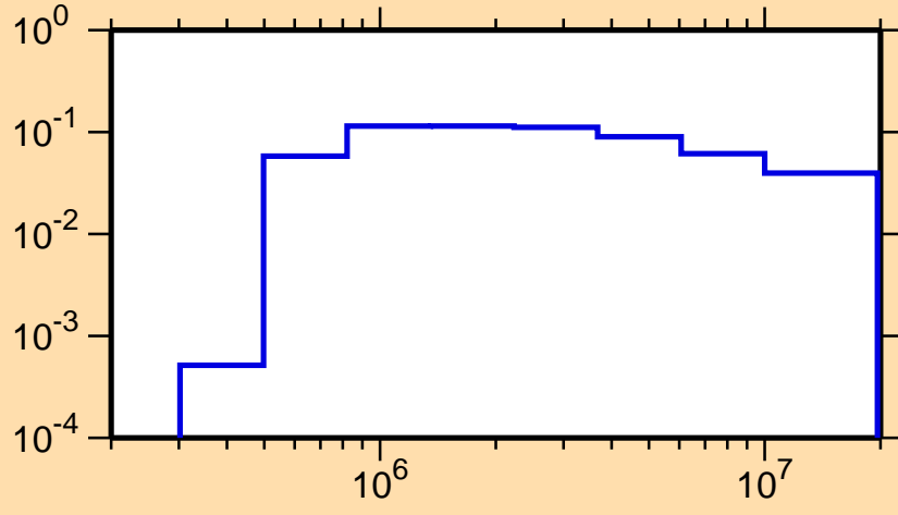
\sigma vs. E for ^{79}\text{Y}(n,n_2)
