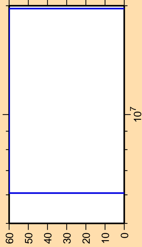
\Delta\sigma/\sigma vs. E for ^{79}\text{Y}(n,\text{pd})
