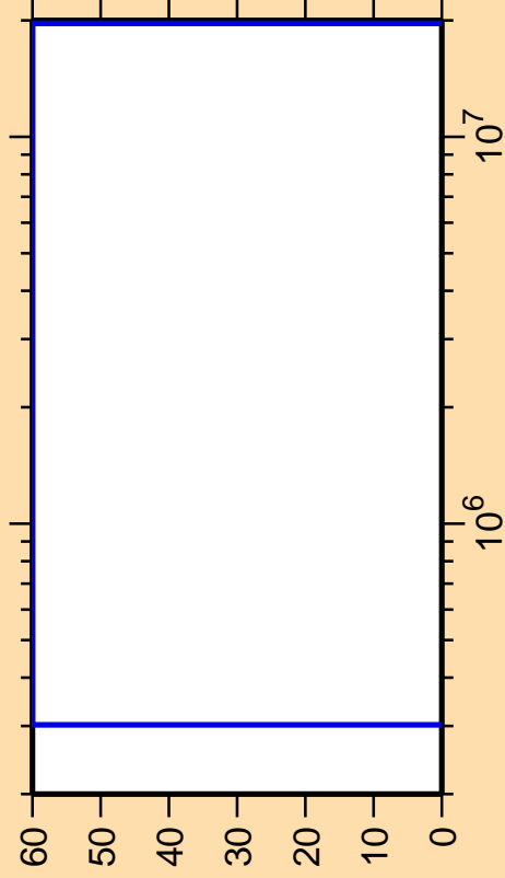
\Delta\sigma/\sigma vs. E for ^{79}\text{Y}(n,n_2)
