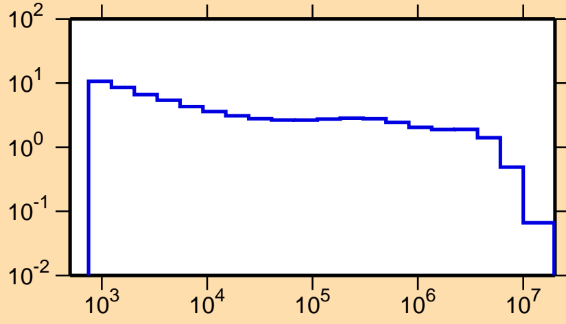
\sigma vs. E for ^{79}\text{Y}(n,p)
