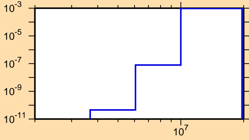
\sigma vs. E for ^{79}\text{Y}(n,\text{He}3)
