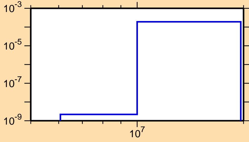
\sigma vs. E for ^{79}\text{Y}(n,n\alpha)
