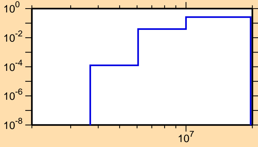
\sigma vs. E for ^{79}\text{Y}(n,np)
