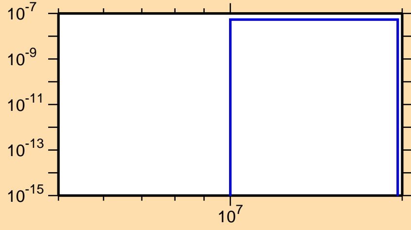
\sigma vs. E for ^{79}\text{Y}(\text{mt117})
