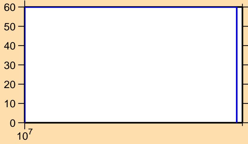
\Delta\sigma/\sigma vs. E for ^{79}\text{Y}(n,\text{inel.})
