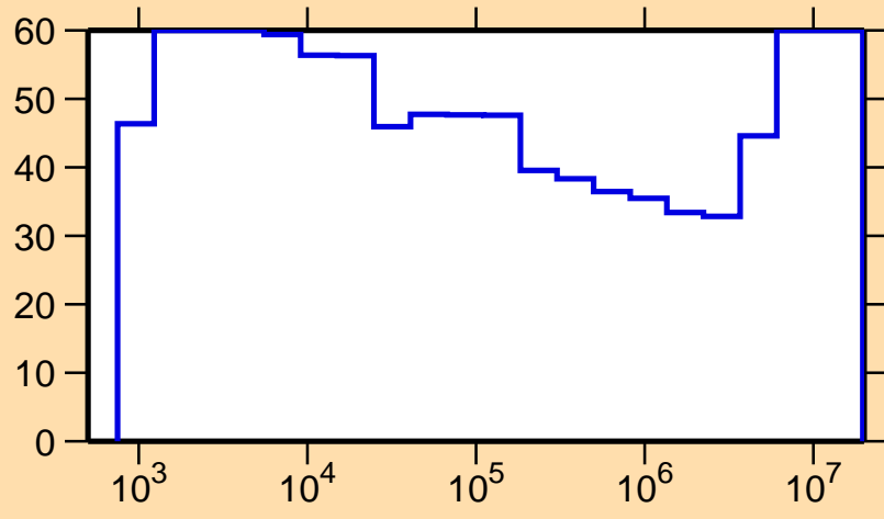
\Delta\sigma/\sigma vs. E for ^{79}\text{Y}(n,p)
