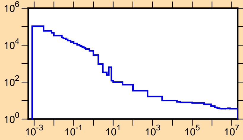
\sigma vs. E for ^{79}\text{Y}(n,\text{tot.})
