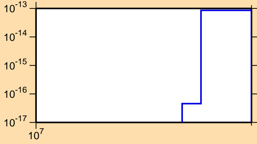
\sigma vs. E for ^{80}\text{Y}(n,2n\alpha)
