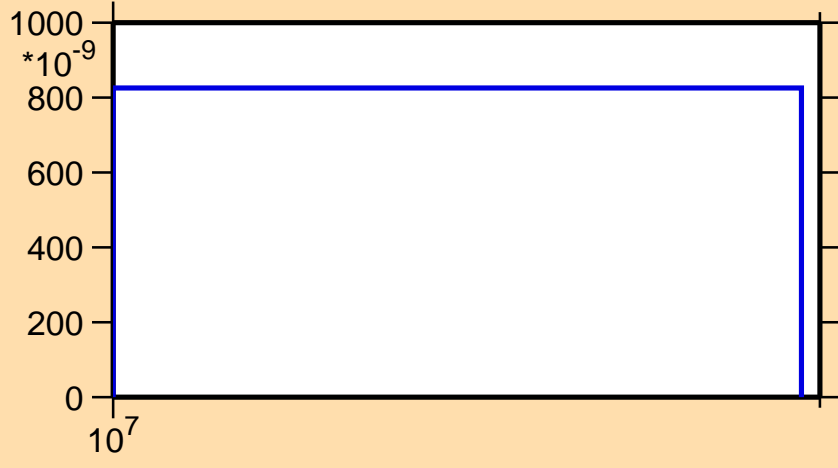
\sigma vs. E for ^{80}\text{Y}(n,pt)
