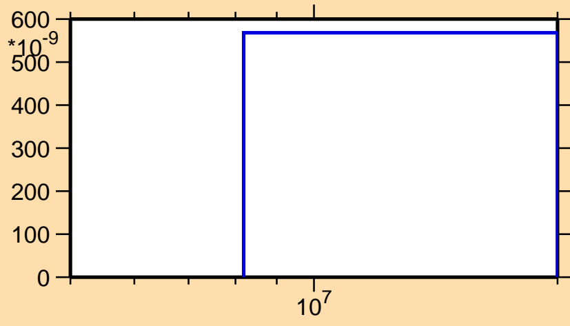
\sigma vs. E for ^{80}\text{Y}(n,\text{nd})
