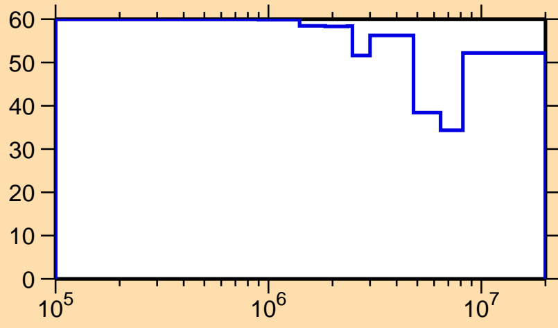
\Delta\sigma/\sigma vs. E for ^{80}\text{Y}(n,n_1)
