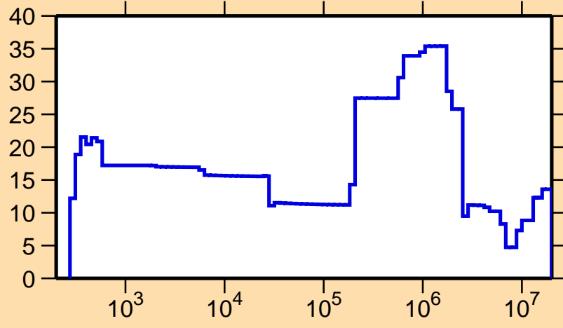
\Delta\sigma/\sigma vs. E for ^{80}\text{Y}(n,el.)
