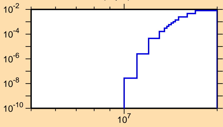
\sigma vs. E for ^{80}\text{Y}(n,\text{pd})
