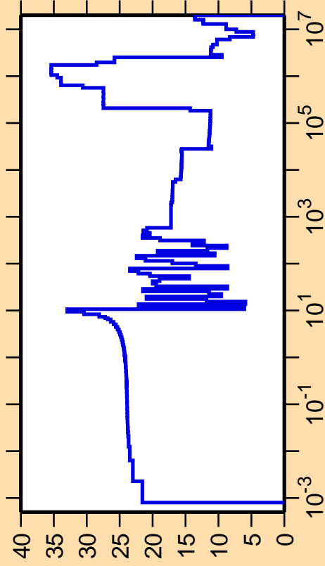
\Delta\sigma/\sigma vs. E for ^{80}\text{Y}(n,\text{el.})
