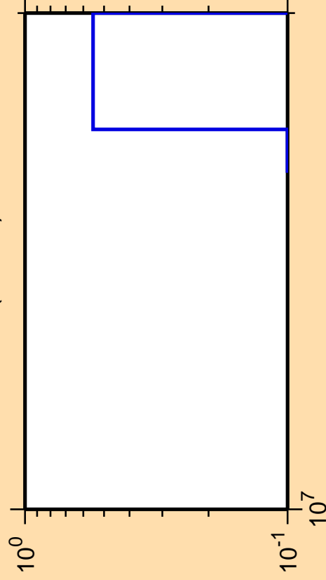
\Delta\sigma/\sigma vs. E for ^{80}\text{Y}(n,2n\alpha)
