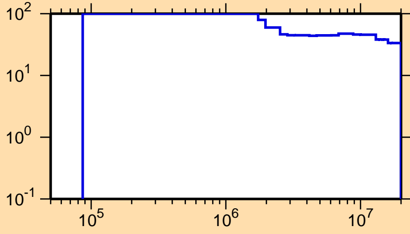
\Delta\sigma/\sigma vs. E for ^{80}\text{Y}(n,n\text{cont.})
