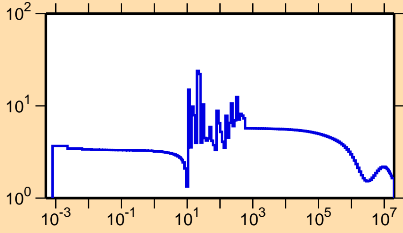
\sigma vs. E for ^{80}\text{Y}(n,\text{el.})
