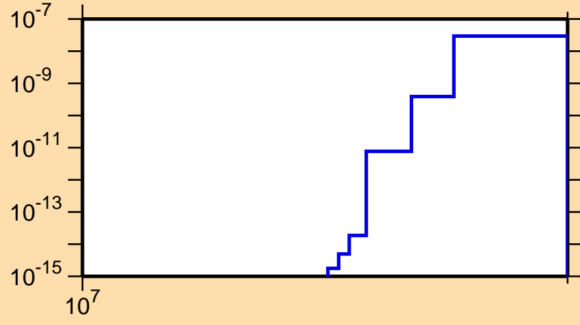
\sigma vs. E for ^{80}\text{Y} (mt 34)
