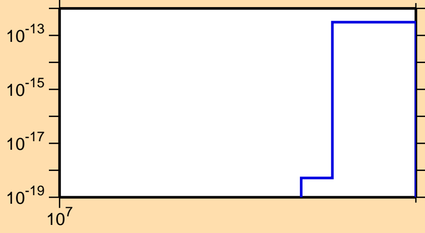
\sigma vs. E for ^{80}\text{Y}(n,2n\alpha)
