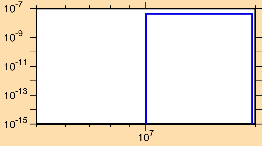
\sigma vs. E for ^{80}\text{Y}(\text{mt117})
