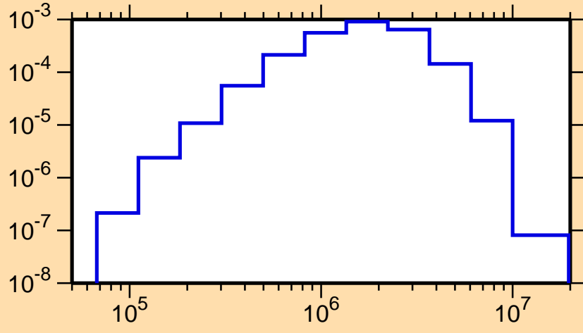
\sigma vs. E for ^{80}\text{Y}(n,n_2)
