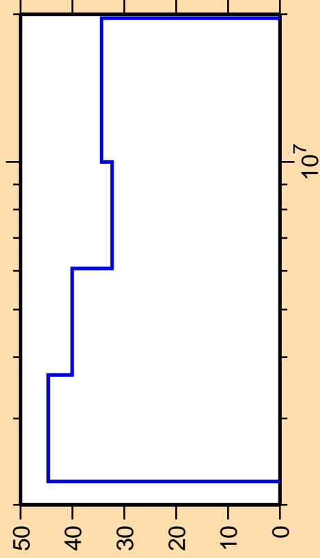
\Delta\sigma/\sigma vs. E for ^{80}\text{Y}(n,np)
