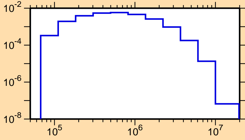
\sigma vs. E for ^{80}\text{Y}(n,n_3)
