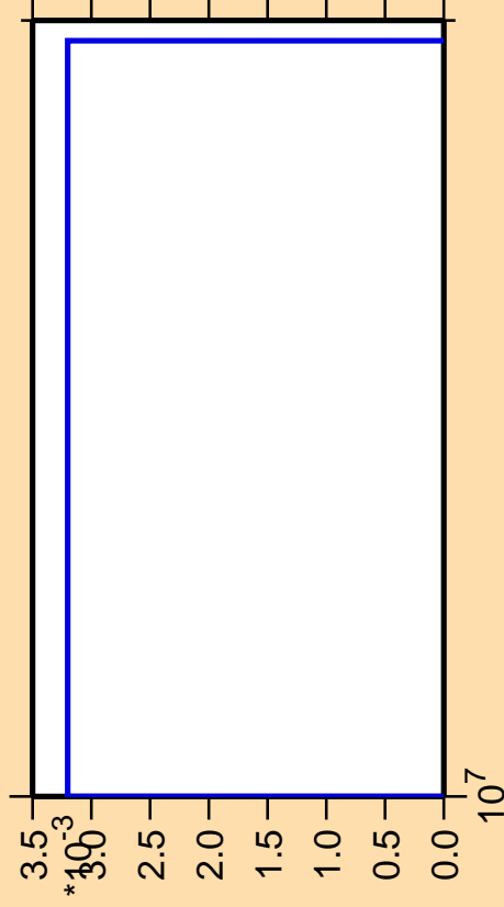
\Delta\sigma/\sigma vs. E for ^{80}\text{Y}(n,2n\alpha)
