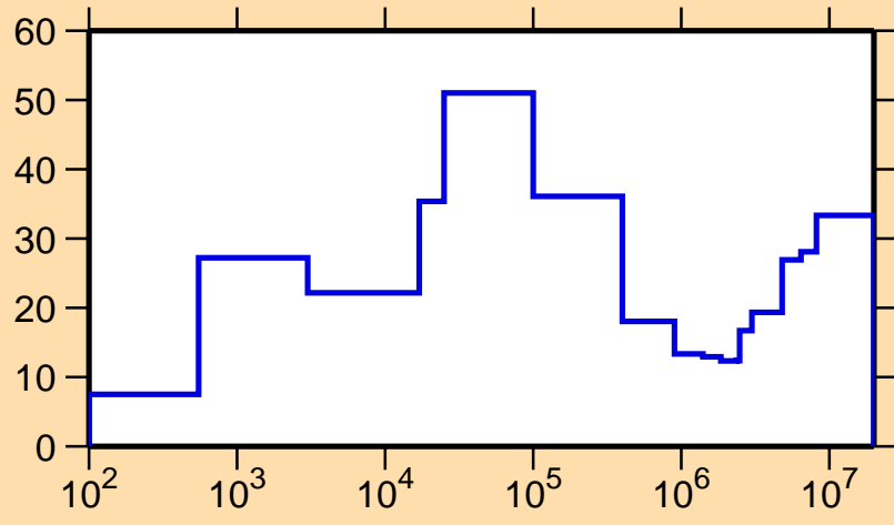
\Delta\sigma/\sigma vs. E for ^{80}\text{Y}(n,p)
