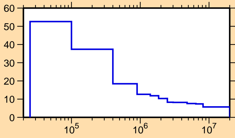
\Delta\sigma/\sigma vs. E for ^{80}\text{Y}(n,n\text{onel.})
