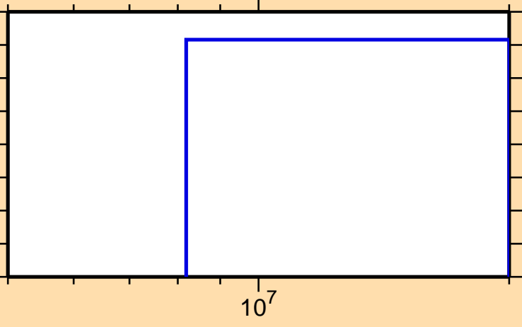
\sigma vs. E for ^{80}\text{Y}(\text{mt117})
