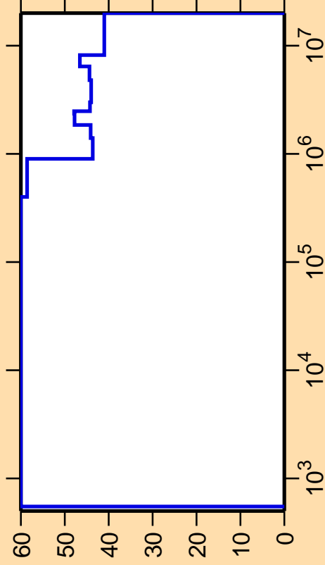
\Delta\sigma/\sigma vs. E for ^{80}\text{Y}(n,\text{inel.})
