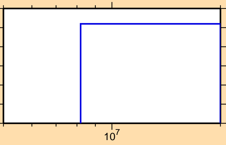
\sigma vs. E for ^{80}\text{Y}(n,2np)
