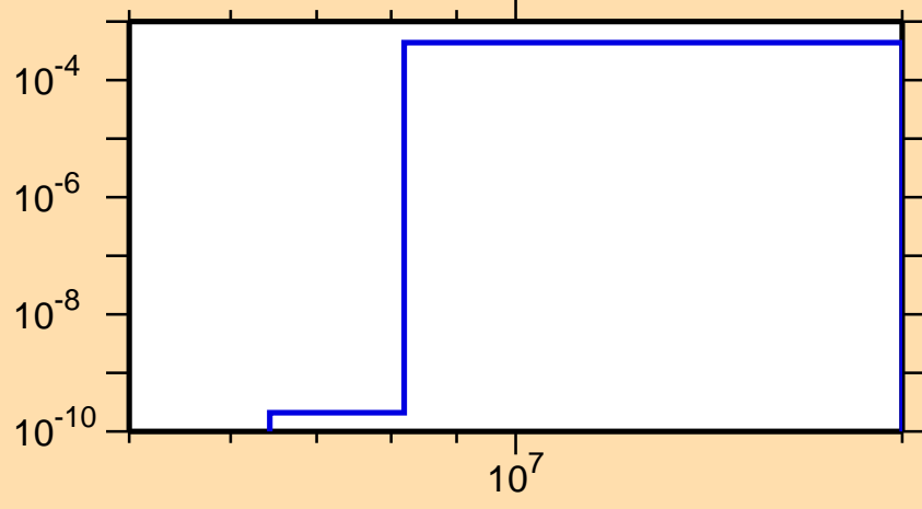
\sigma vs. E for ^{80}\text{Y}(n,t)
