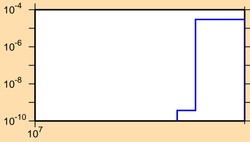
\sigma vs. E for ^{81}\text{Y}(n,2np)
