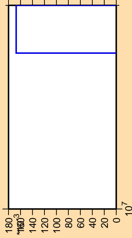
\Delta\sigma/\sigma vs. E for ^{81}\text{Y}(n,nt)
