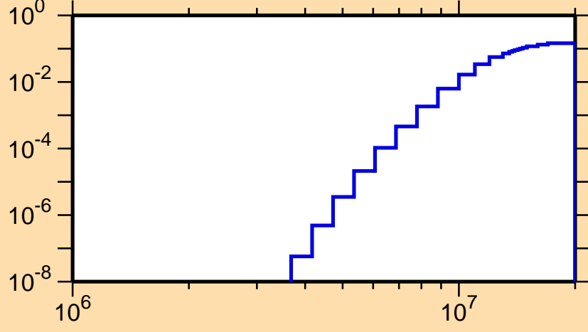
\sigma vs. E for ^{81}\text{Y}(n,p\alpha)
