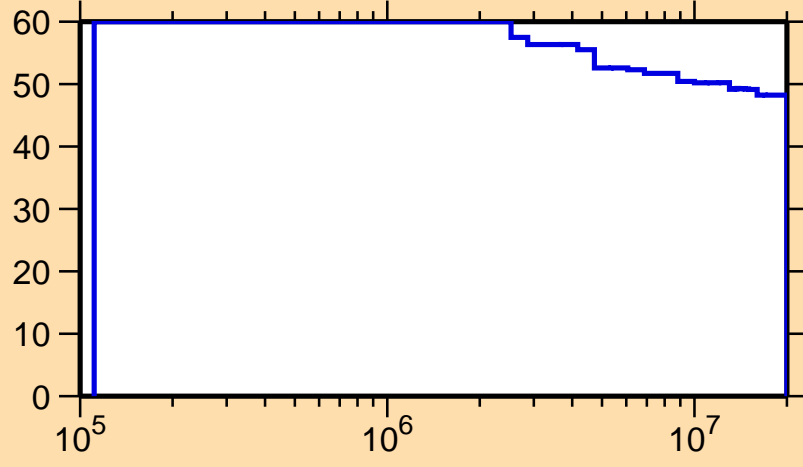
\Delta\sigma/\sigma vs. E for ^{81}\text{Y}(n,n_1)
