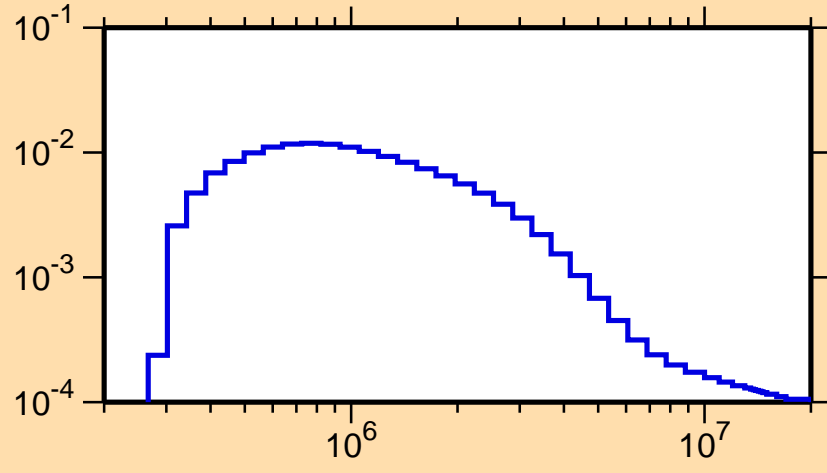
\sigma vs. E for ^{81}\text{Y}(n,n_4)
