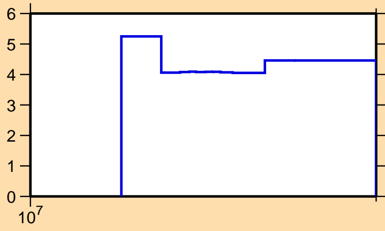
\Delta\sigma/\sigma vs. E for ^{81}\text{Y}(n,\text{tot.})
