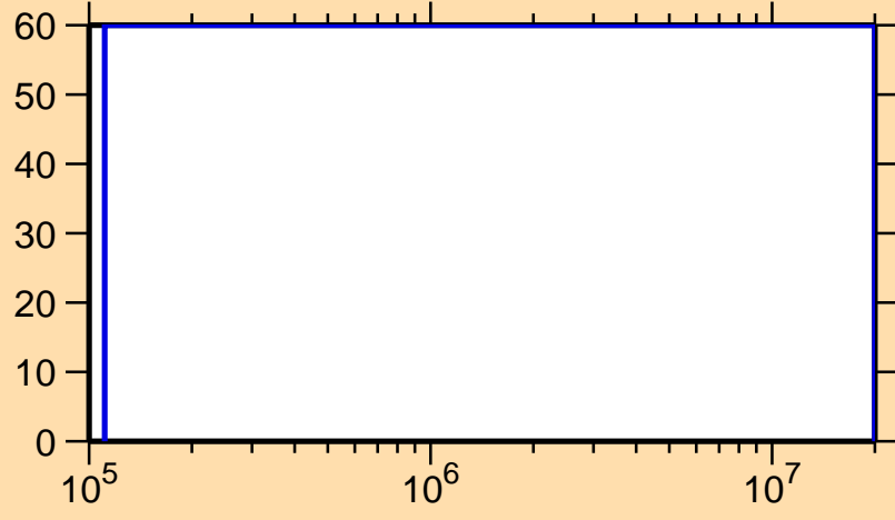
\Delta\sigma/\sigma vs. E for ^{81}\text{Y}(n,\text{inel.})
