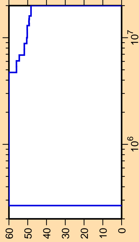
\Delta\sigma/\sigma vs. E for ^{81}\text{Y}(n,n_3)
