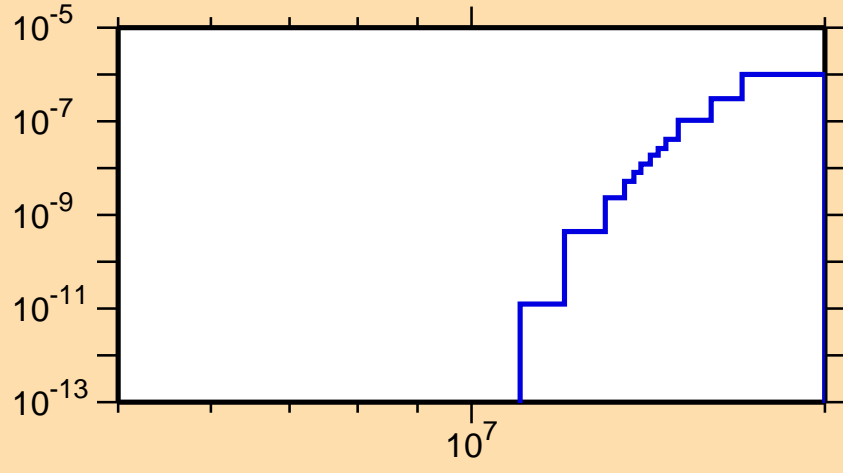
\sigma vs. E for ^{81}\text{Y}(\text{mt117})
