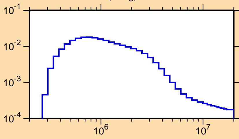
\sigma vs. E for ^{81}\text{Y}(n,n_3)
