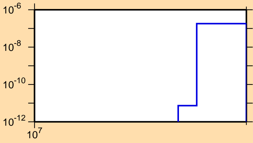
\sigma vs. E for ^{81}\text{Y}(n,\text{pt})
