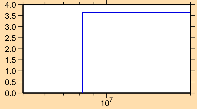
\Delta\sigma/\sigma vs. E for ^{81}\text{Y}(n,\text{tot.})
