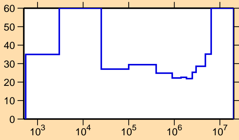
\Delta\sigma/\sigma vs. E for ^{81}\text{Y}(n,p)
