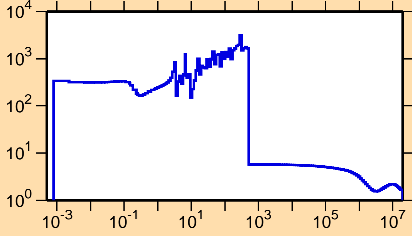
\sigma vs. E for ^{82}\text{Y}(n,\text{el.})
