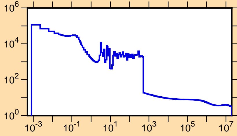
\sigma vs. E for ^{82}\text{Y}(n,\text{tot.})
