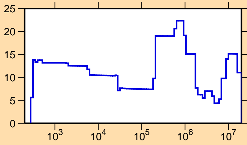
\Delta\sigma/\sigma vs. E for ^{82}\text{Y}(n,el.)
