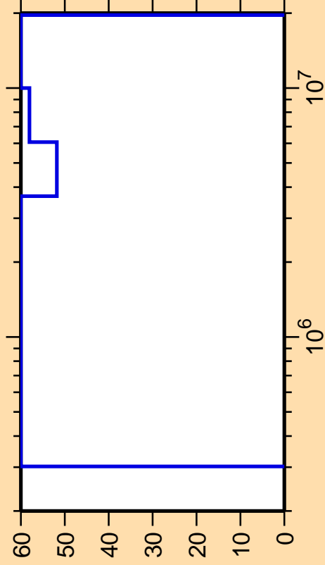
\Delta\sigma/\sigma vs. E for ^{82}\text{Y}(n,n_3)
