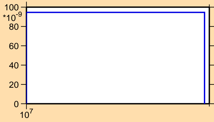
\sigma vs. E for ^{82}\text{Y}(n,\text{pt})
