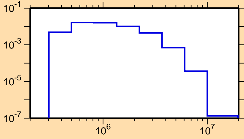
\sigma vs. E for ^{82}\text{Y}(n,n_3)
