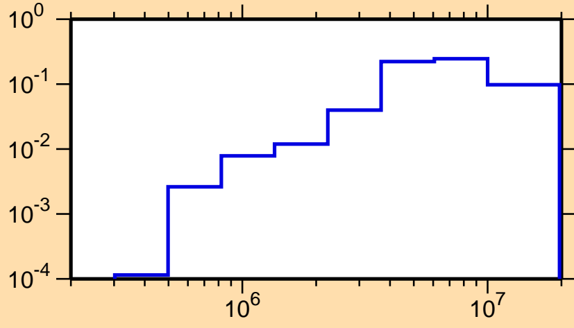
\sigma vs. E for ^{82}\text{Y}(n,n\text{cont.})
