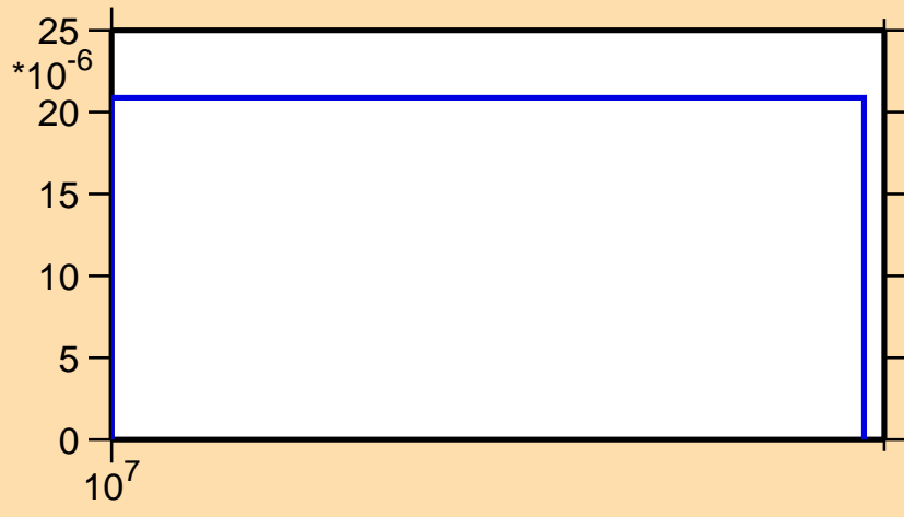
\sigma vs. E for ^{82}\text{Y}(n,nd)
