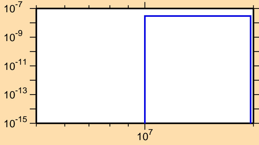
\sigma vs. E for ^{82}\text{Y}(\text{mt117})
