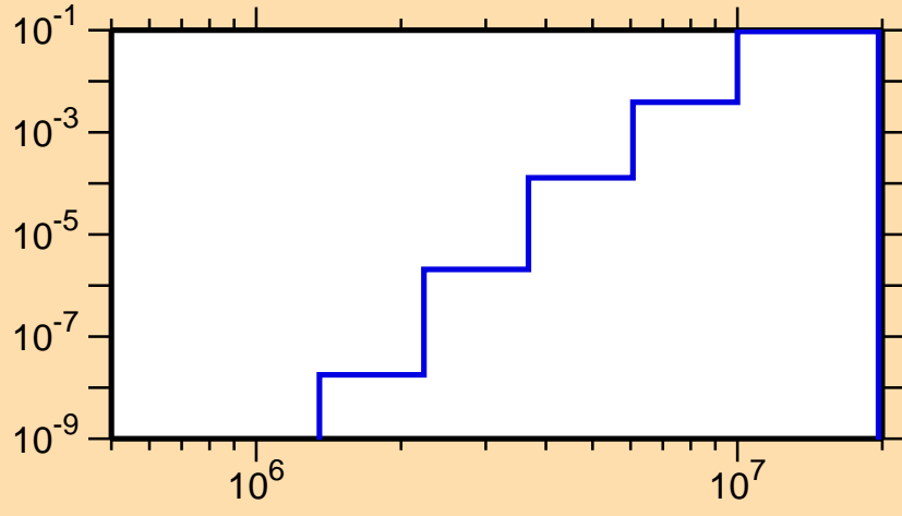
\sigma vs. E for ^{82}\text{Y}(n,p\alpha)
