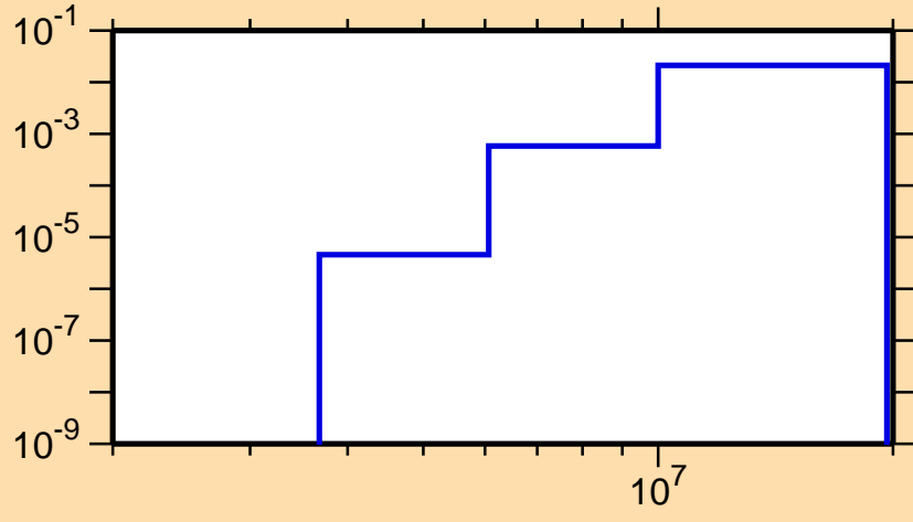
\sigma vs. E for ^{82}\text{Y}(n,d)
