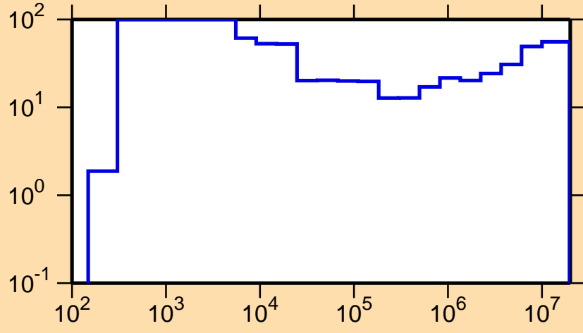
\Delta\sigma/\sigma vs. E for ^{82}\text{Y}(n,p)
