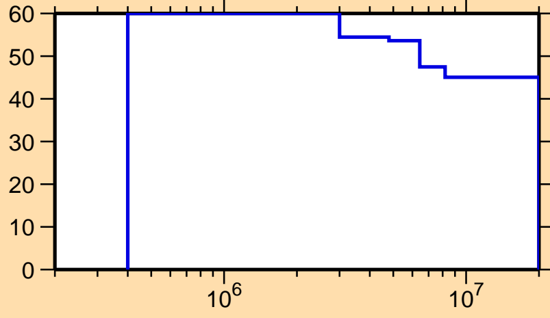
\Delta\sigma/\sigma vs. E for ^{82}\text{Y}(n,ncont.)
