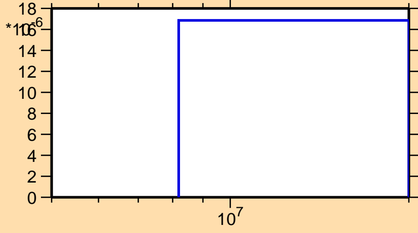
\sigma vs. E for ^{82}\text{Y}(n,\text{nd})
