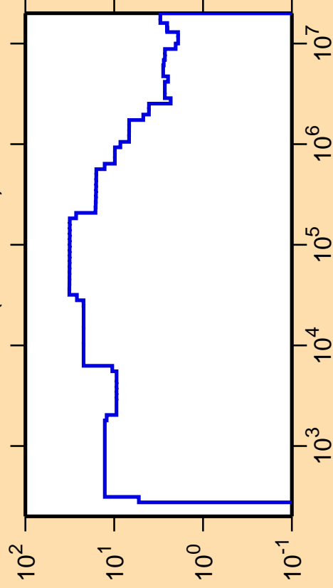
\Delta\sigma/\sigma vs. E for ^{83}\text{Y}(n,\text{nonel.})
