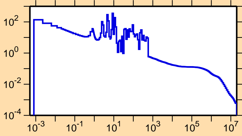
\sigma vs. E for ^{83}\text{Y}(n,\gamma)
