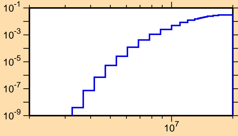
\sigma vs. E for ^{83}\text{Y}(n,d)
