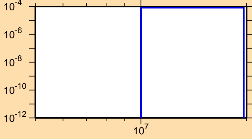
\sigma vs. E for ^{83}\text{Y}(n,t)
