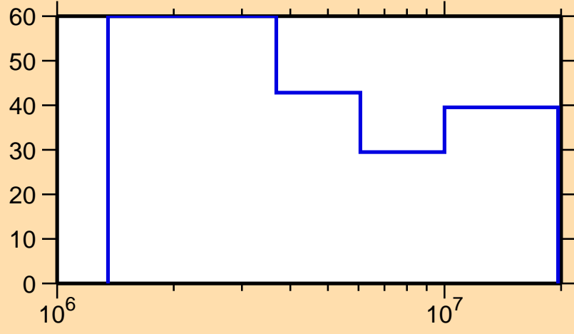
\Delta\sigma/\sigma vs. E for ^{83}\text{Y}(n,n\text{cont.})
