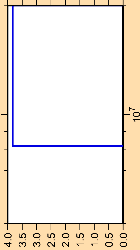
\Delta\sigma/\sigma vs. E for ^{83}\text{Y}(n,nt)
