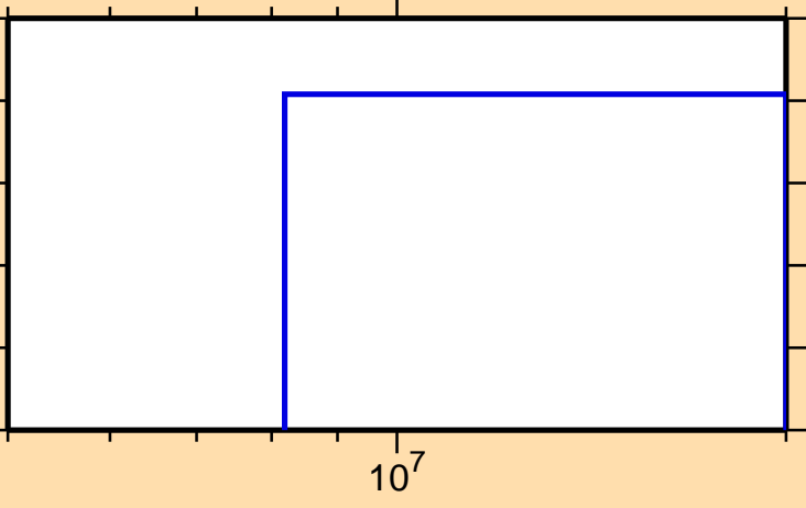
\sigma vs. E for ^{83}\text{Y}(n,\text{nd})
