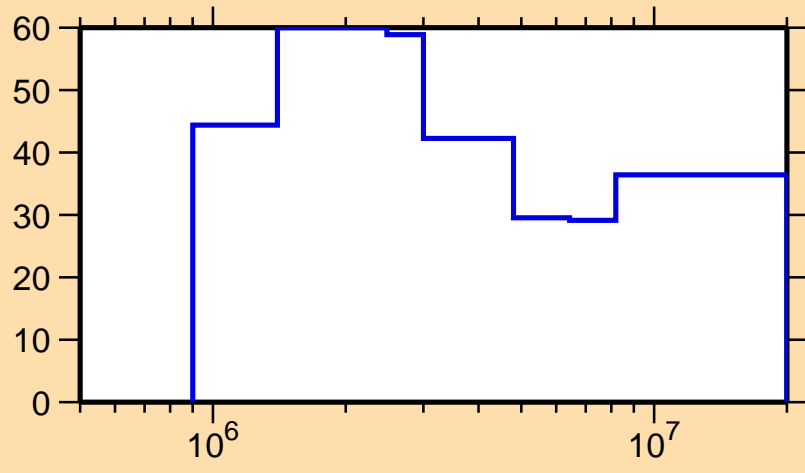
\Delta\sigma/\sigma vs. E for ^{83}\text{Y}(n,n\text{cont.})
