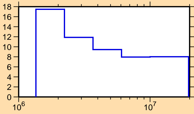
\Delta\sigma/\sigma vs. E for ^{84}\text{Y}(n,n\text{onel.})
