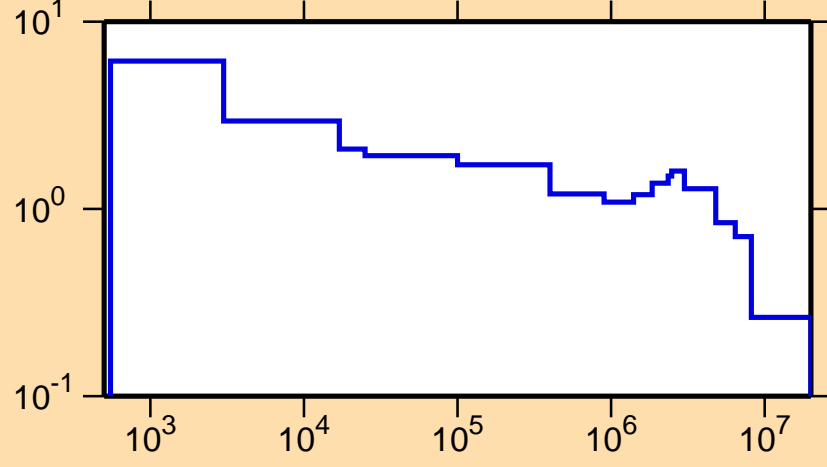
\sigma vs. E for ^{84}\text{Y}(n,p)
