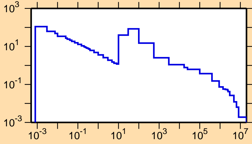
\sigma vs. E for ^{85}\text{Y}(n,\gamma)
