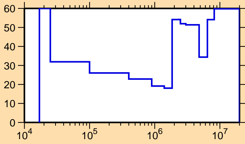
\Delta\sigma/\sigma vs. E for ^{85}\text{Y}(n,n_1)
