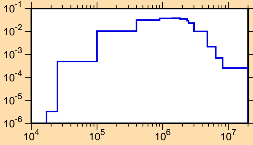
\sigma vs. E for ^{85}\text{Y}(n,n_1)
