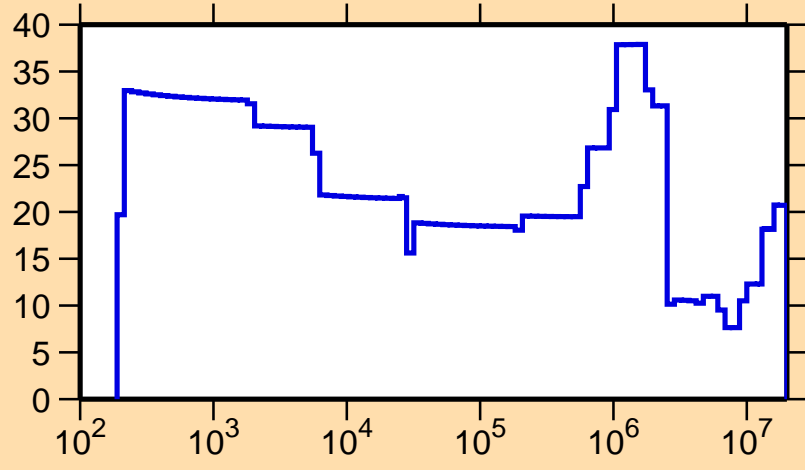
\Delta\sigma/\sigma vs. E for ^{85}\text{Y}(n,el.)
