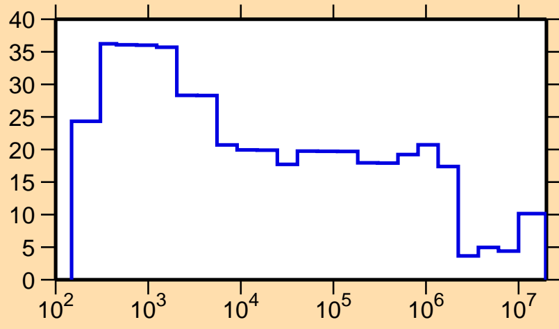
\Delta\sigma/\sigma vs. E for ^{85}\text{Y}(n,\text{tot.})
