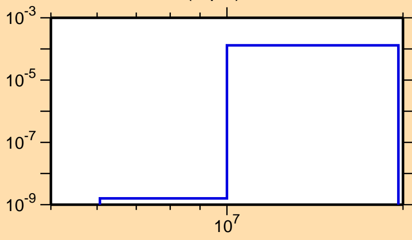
\sigma vs. E for ^{85}\text{Y}(n,p\alpha)
