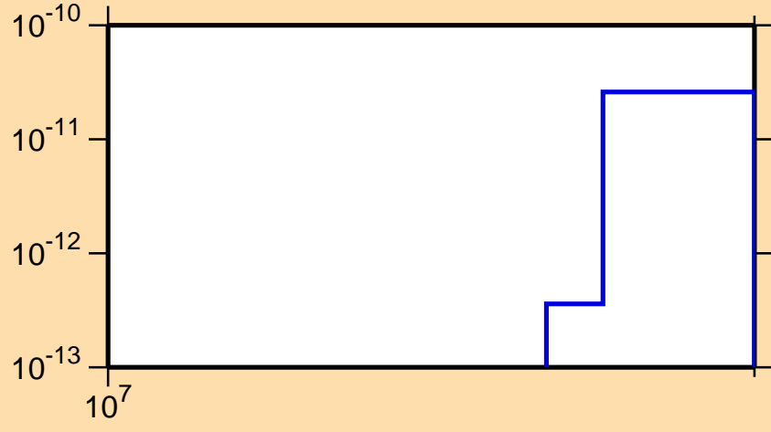
\sigma vs. E for ^{86}\text{Y}(\text{mt117})
