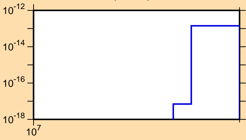
\sigma vs. E for ^{86}\text{Y} (mt 34)
