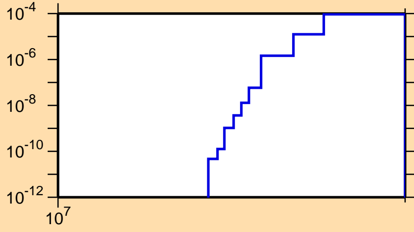
\sigma vs. E for ^{86}\text{Y}(n,\text{nd})
