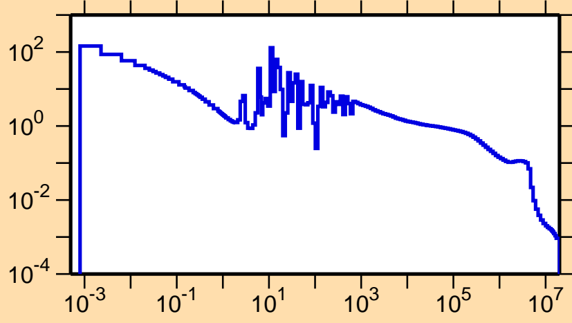
\sigma vs. E for ^{86}\text{Y}(n,\gamma)
