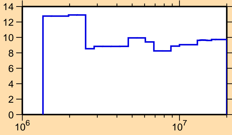
\Delta\sigma/\sigma vs. E for ^{86}\text{Y}(n,n\text{onel.})
