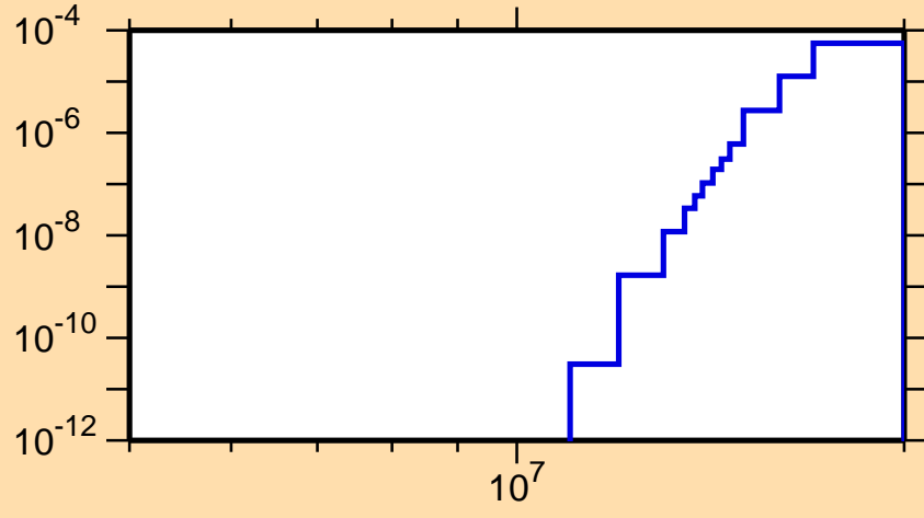
\sigma vs. E for ^{86}\text{Y}(n,\text{He}3)
