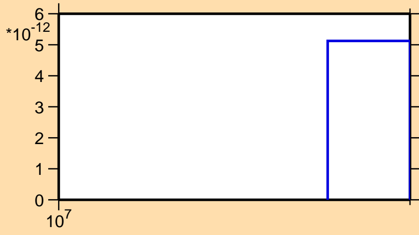
\sigma vs. E for ^{86}\text{Y}(n,nt)
