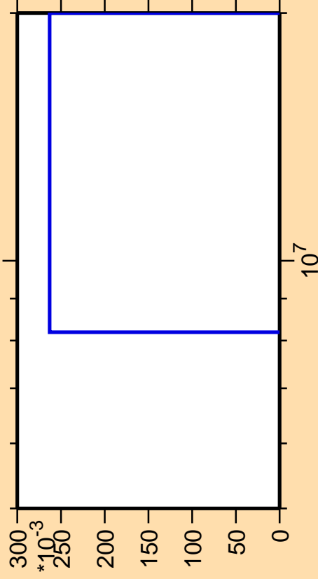
\Delta\sigma/\sigma vs. E for ^{86}\text{Y}(n,nt)
