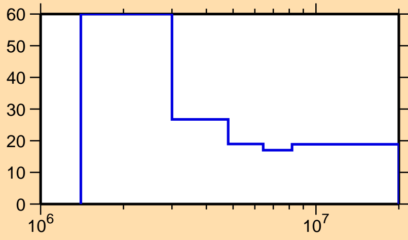
\Delta\sigma/\sigma vs. E for ^{86}\text{Y}(n,n\text{cont.})
