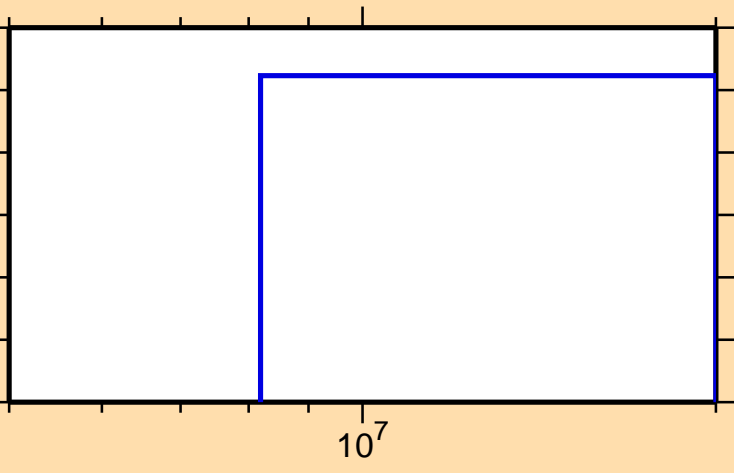
\sigma vs. E for ^{86}\text{Y}(n,2n\alpha)
